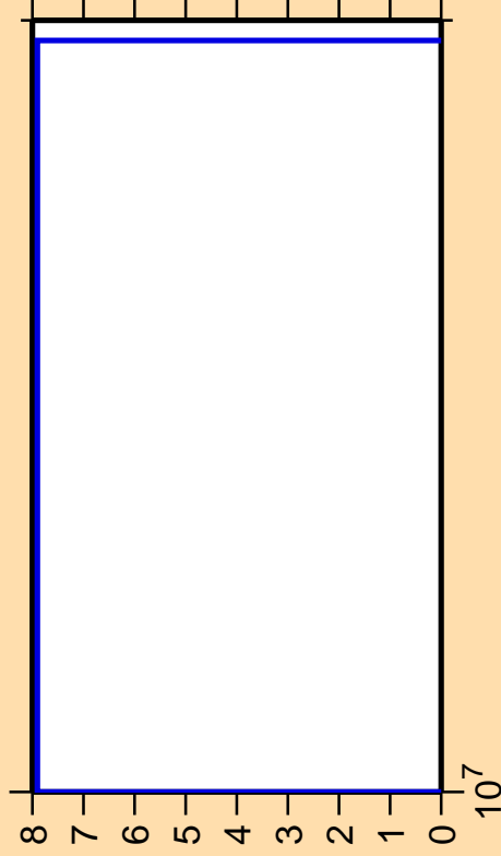
\Delta\sigma/\sigma vs. E for ^{179}\text{Hf}(n,3n)
