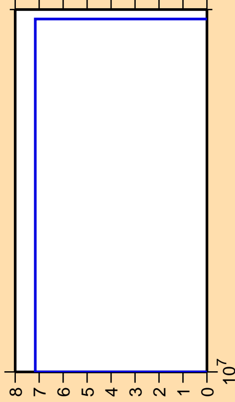
\Delta\sigma/\sigma vs. E for ^{179}\text{Hf}(n,\text{He3})
