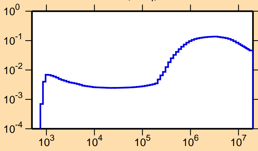
\sigma vs. E for ^{179}\text{Hf}(n,n_4)
