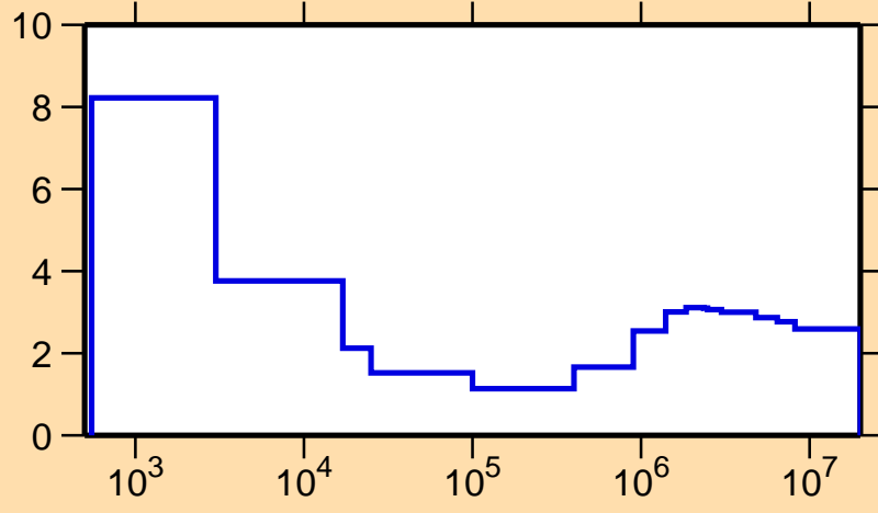
\sigma vs. E for ^{179}\text{Hf}(n,\text{nonel.})
