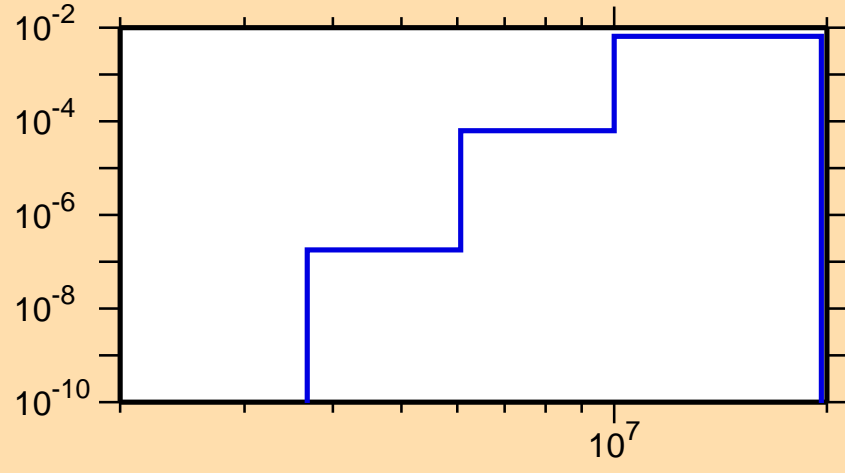
\sigma vs. E for ^{179}\text{Hf}(n,p)
