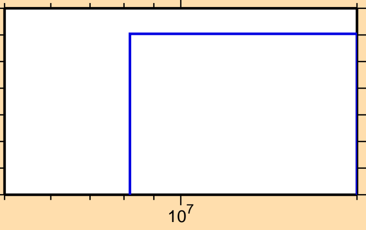
\sigma vs. E for ^{179}\text{Hf}(n,nt)
