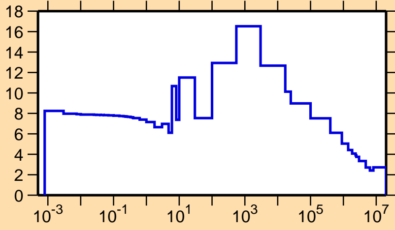
\sigma vs. E for ^{179}\text{Hf}(n,\text{el.})
