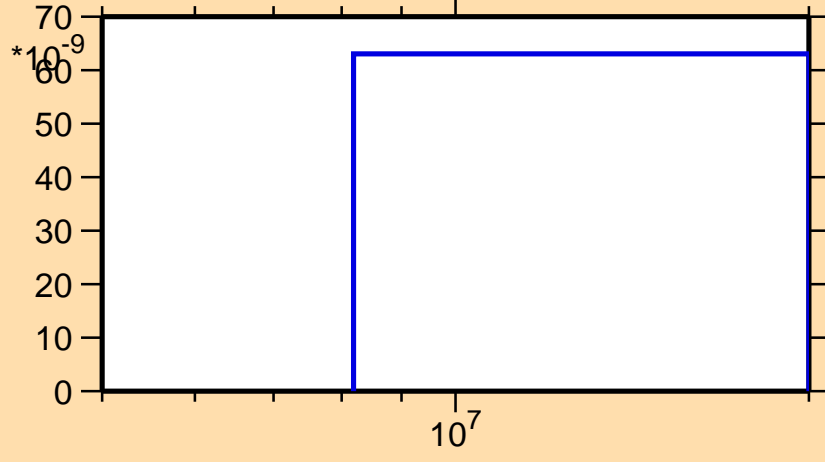
\sigma vs. E for ^{179}\text{Hf}(n,nd)
