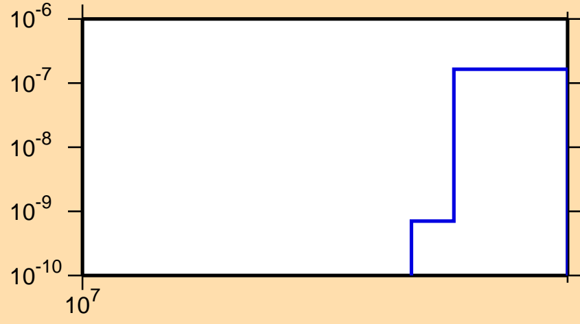
\sigma vs. E for ^{180}\text{Hf}(n,nd)
