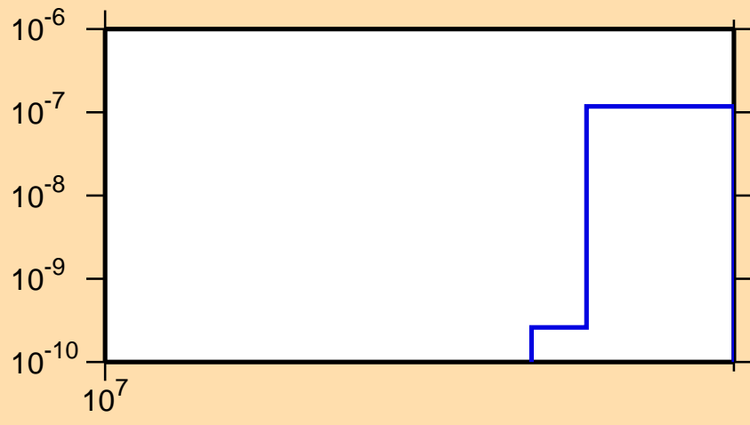
\sigma vs. E for ^{180}\text{Hf}(n,nt)
