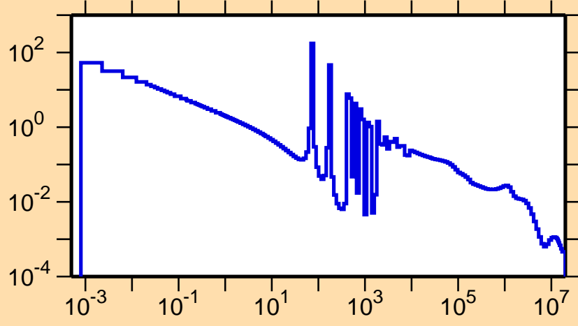
\sigma vs. E for ^{180}\text{Hf}(n,\gamma)
