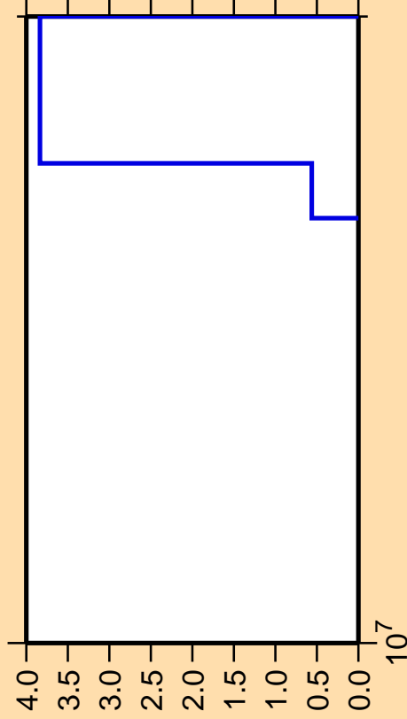
\Delta\sigma/\sigma vs. E for ^{180}\text{Hf}(n,p\alpha)
