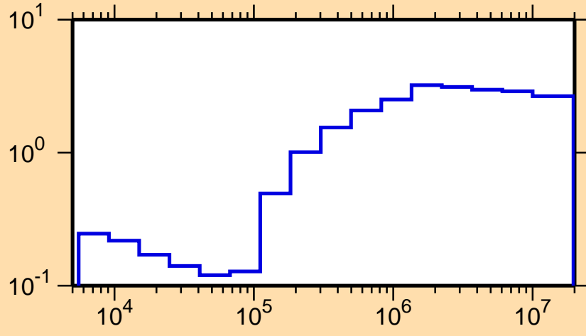
\sigma vs. E for ^{180}\text{Hf}(n,\text{nonel.})
