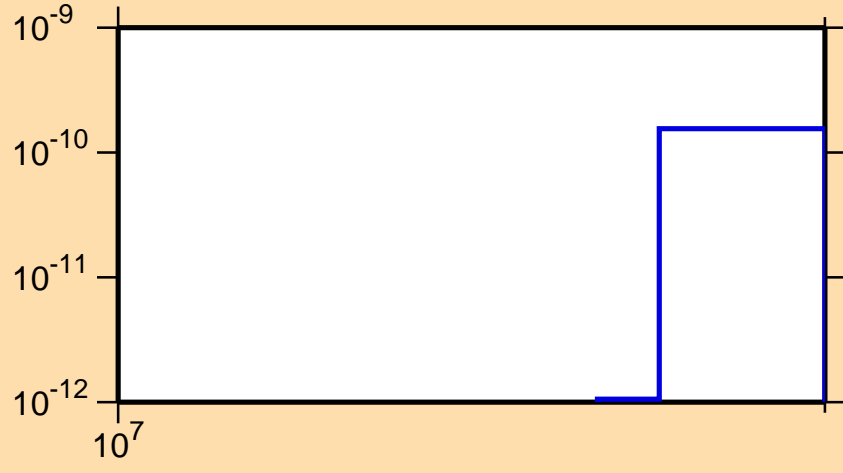
\sigma vs. E for ^{180}\text{Hf}(n,3n\alpha)
