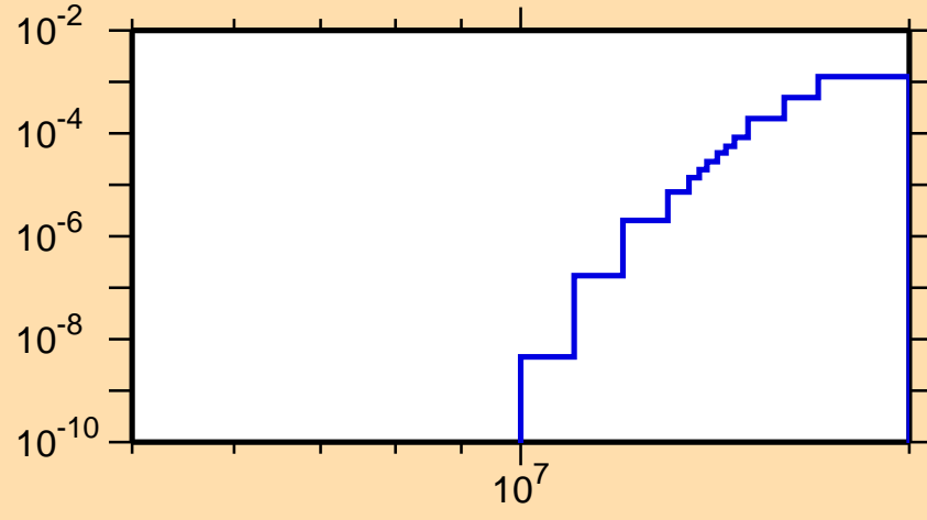
\sigma vs. E for ^{180}\text{Hf}(n,np)
