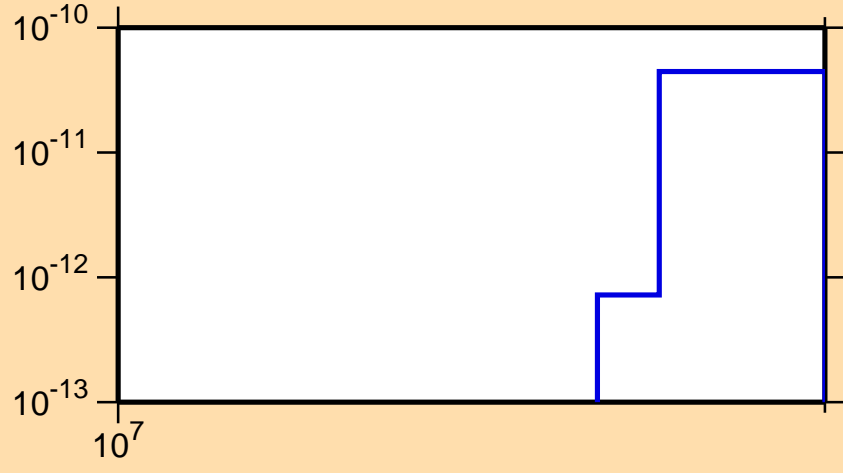
\sigma vs. E for ^{180}\text{Hf}(n,\text{He3})
