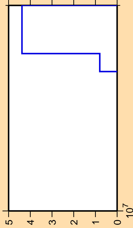
\Delta\sigma/\sigma vs. E for ^{180}\text{Hf}(n,p\alpha)
