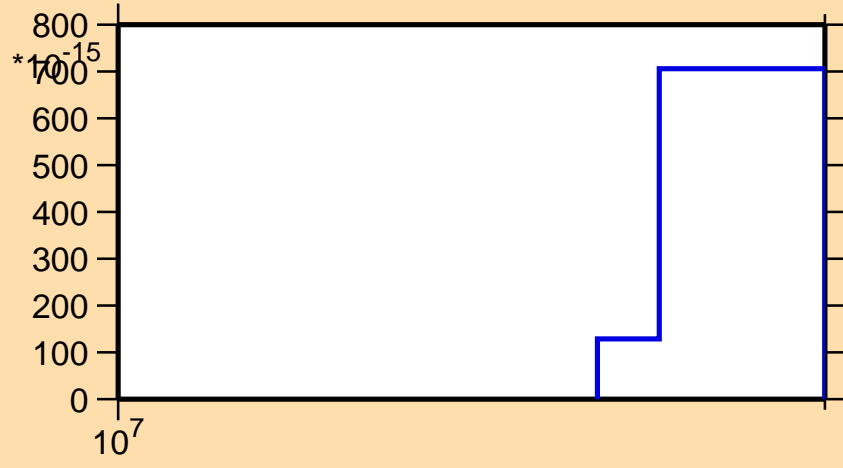
\sigma vs. E for ^{180}\text{Hf}(n,p\alpha)
