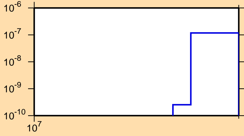
\sigma vs. E for ^{180}\text{Hf}(n,2np)
