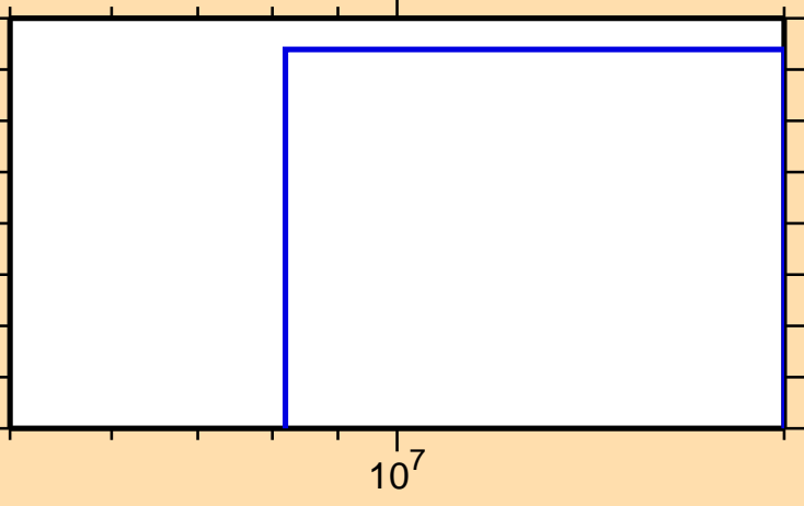
\sigma vs. E for ^{180}\text{Hf}(n,p\alpha)
