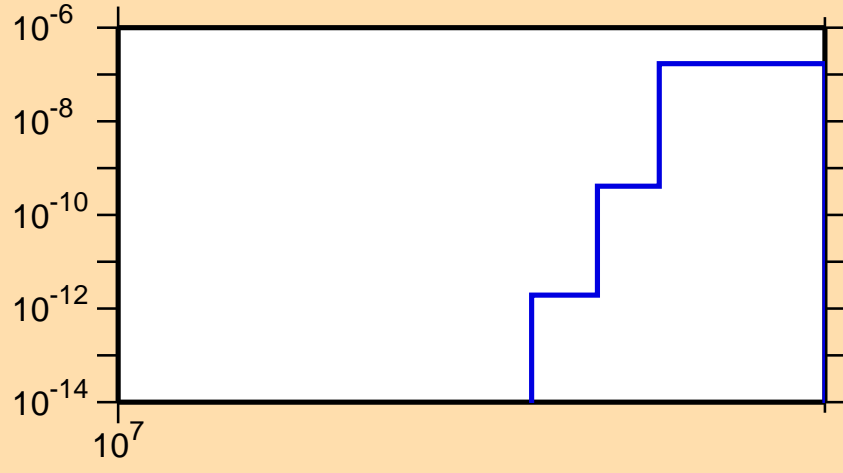
\sigma vs. E for ^{181}\text{Hf}(n,2np)
