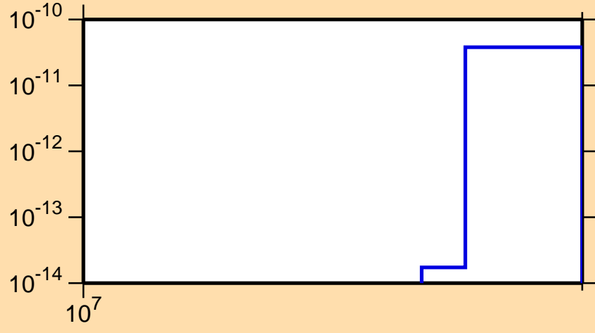
\sigma vs. E for ^{181}\text{Hf}(n,3n\alpha)
