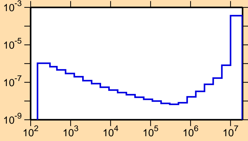
\sigma vs. E for ^{181}\text{Hf}(n,\alpha)
