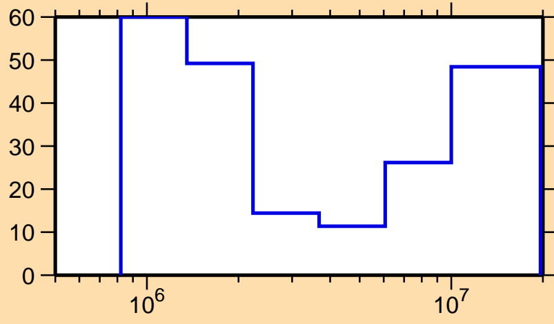
\Delta\sigma/\sigma vs. E for ^{181}\text{Hf}(n,n\text{cont.})
