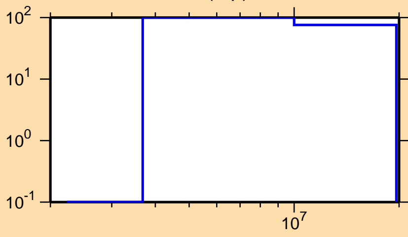
\Delta\sigma/\sigma vs. E for ^{181}\text{Hf}(n,p)
