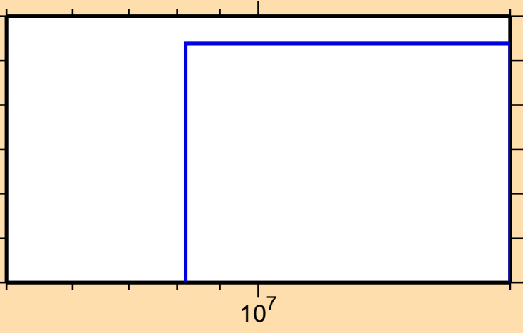
\sigma vs. E for ^{181}\text{Hf}(n,\text{nd})
