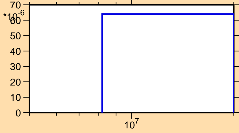
\sigma vs. E for ^{181}\text{Hf}(n,np)
