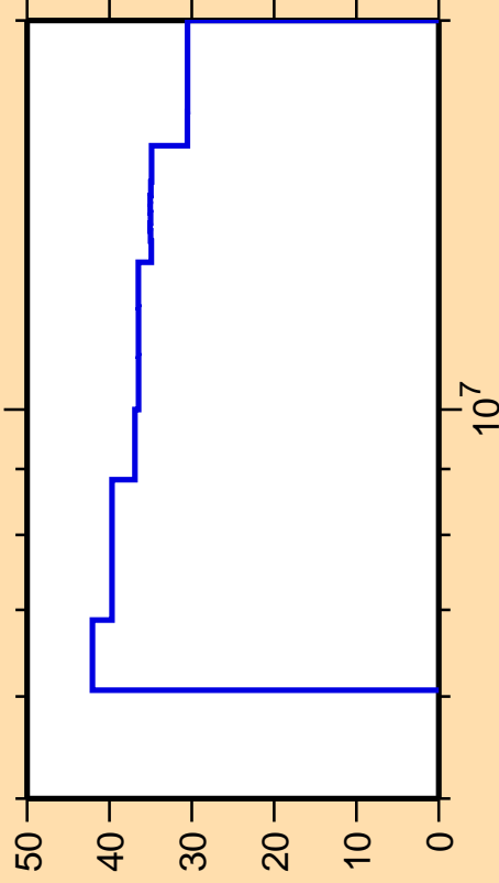
\Delta\sigma/\sigma vs. E for ^{182}\text{Hf}(n,n_1)
