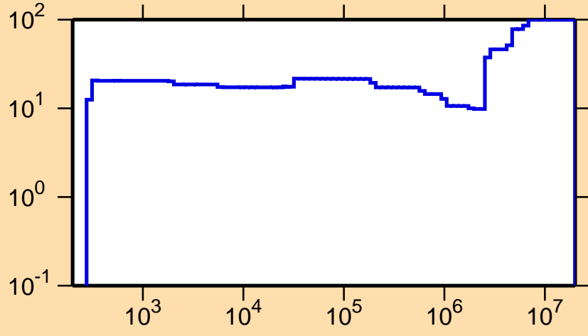
\Delta\sigma/\sigma vs. E for ^{182}\text{Hf}(n,\gamma)
