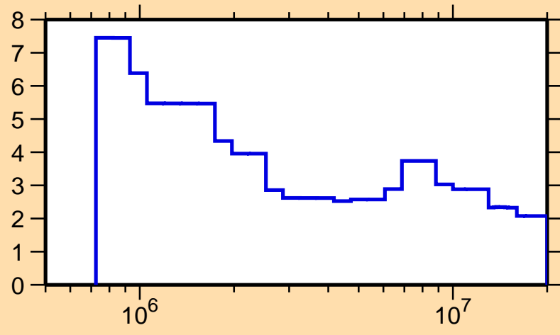
\Delta\sigma/\sigma vs. E for ^{182}\text{Hf}(n,n\text{oncl.})
