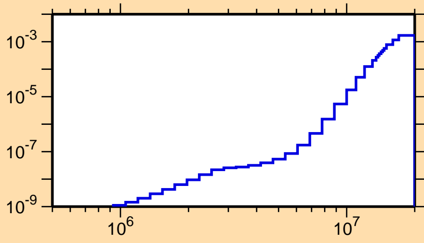
\sigma vs. E for ^{182}\text{Hf}(n,\alpha)
