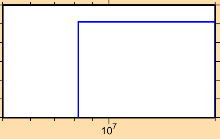
\sigma vs. E for ^{182}\text{Hf}(n,2n\alpha)
