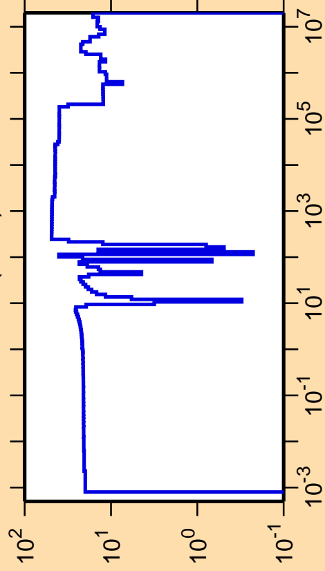
\Delta\sigma/\sigma vs. E for ^{183}\text{Hf}(n,\text{el.})
