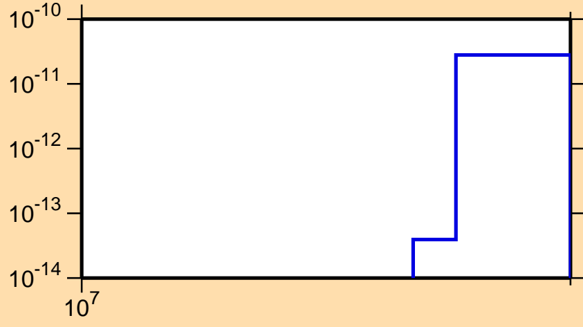
\sigma vs. E for ^{183}\text{Hf}(n,3n\alpha)
