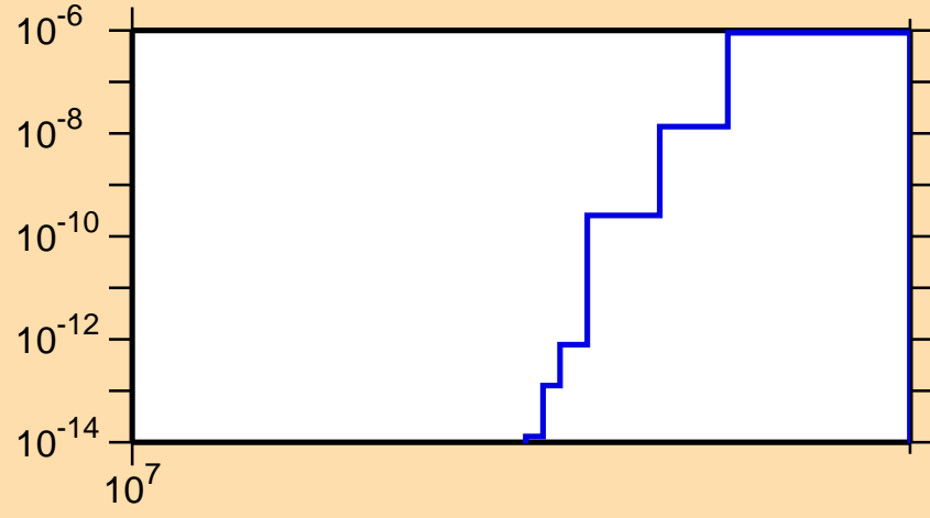
\sigma vs. E for ^{183}\text{Hf}(n,\text{nd})
