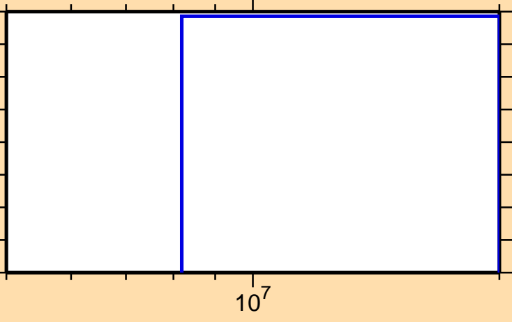
\sigma vs. E for ^{183}\text{Hf}(n,\text{nd})
