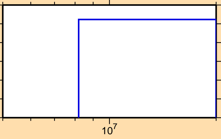
\sigma vs. E for ^{183}\text{Hf}(n,nt)
