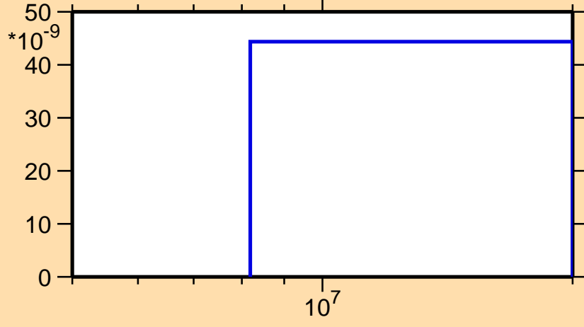
\sigma vs. E for ^{183}\text{Hf}(n,2n\alpha)
