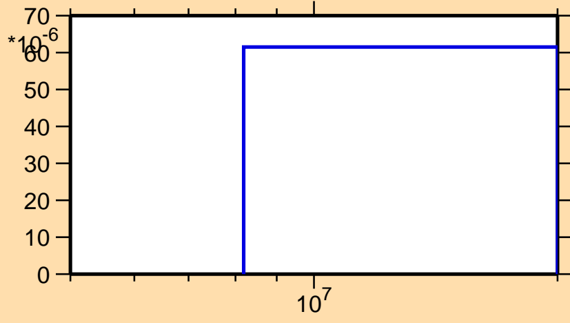
\sigma vs. E for ^{183}\text{Hf}(n,d)
