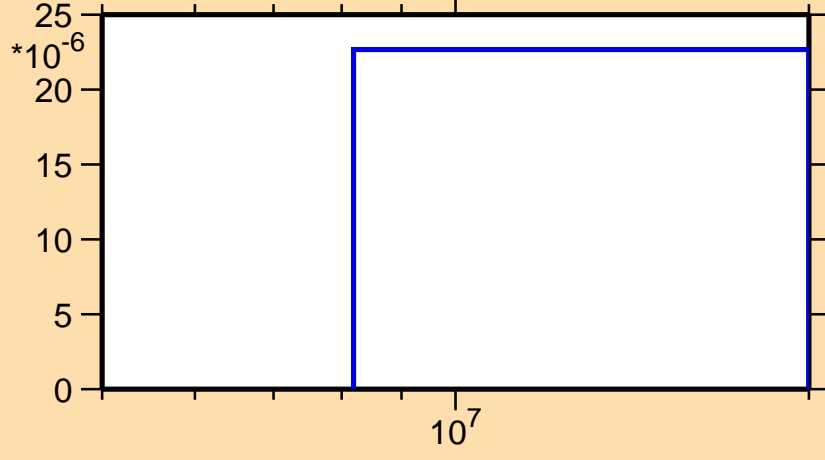
\sigma vs. E for ^{183}\text{Hf}(n,np)
