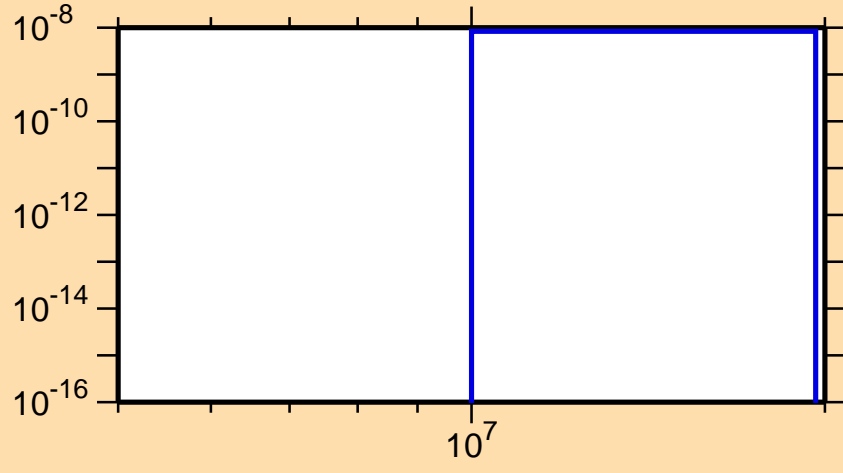
\sigma vs. E for ^{184}\text{Hf}(n,2n\alpha)
