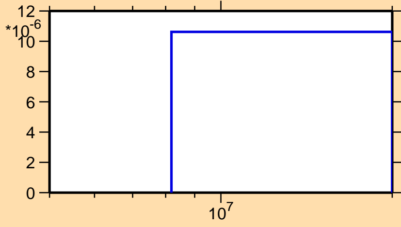
\sigma vs. E for ^{184}\text{Hf}(n,np)
