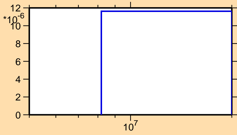
\sigma vs. E for ^{184}\text{Hf}(n,t)
