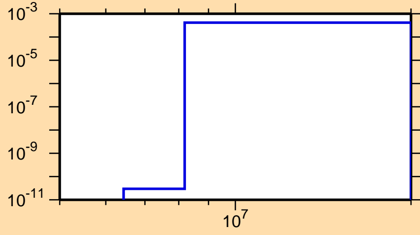
\sigma vs. E for ^{184}\text{Hf}(n,p)
