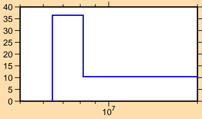
\Delta\sigma/\sigma vs. E for ^{184}\text{Hf}(n,el.)
