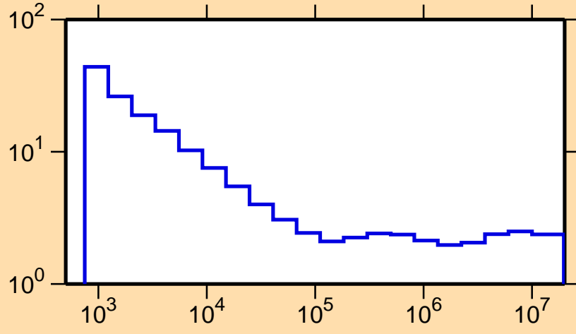
\sigma vs. E for ^{184}\text{Hf}(n,\text{nonel.})
