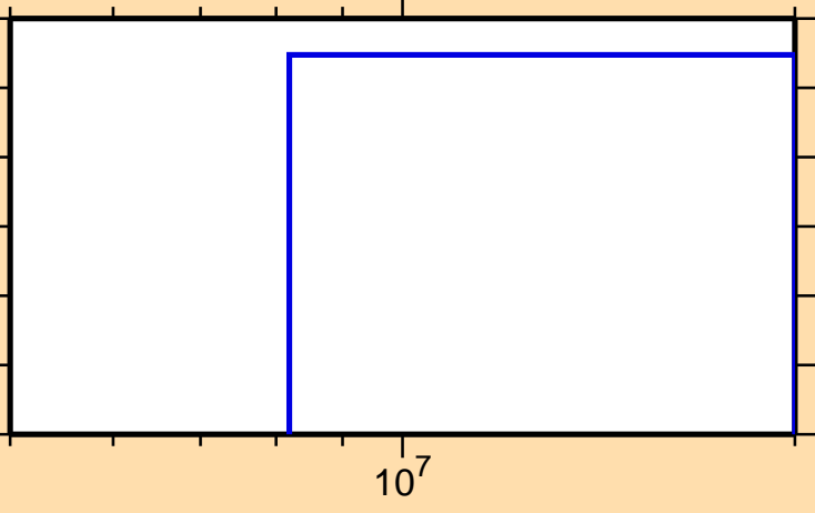
\sigma vs. E for ^{184}\text{Hf}(n,\text{nd})
