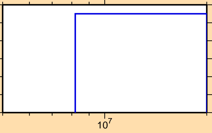
\sigma vs. E for ^{184}\text{Hf}(n,np)
