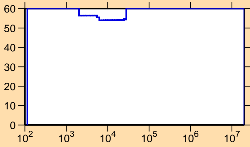
\Delta\sigma/\sigma vs. E for ^{185}\text{Hf}(n,\gamma)
