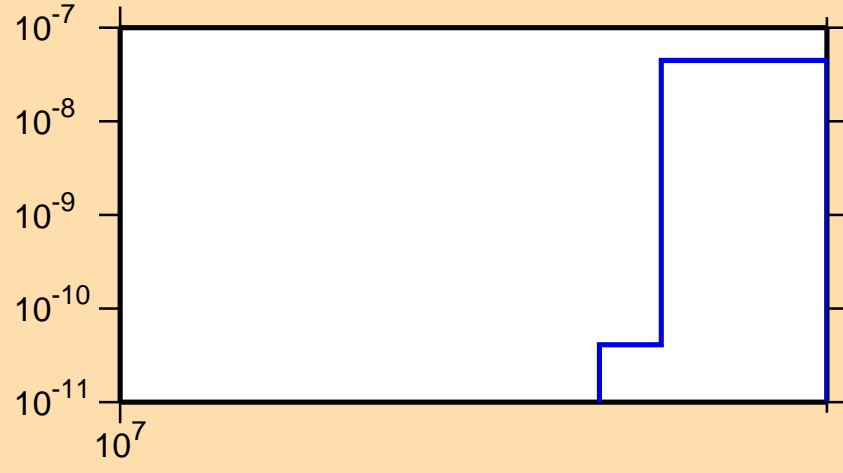
\sigma vs. E for ^{185}\text{Hf}(n,2np)
