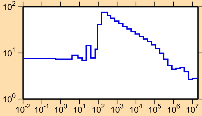
\sigma vs. E for ^{185}\text{Hf}(n,\text{el.})
