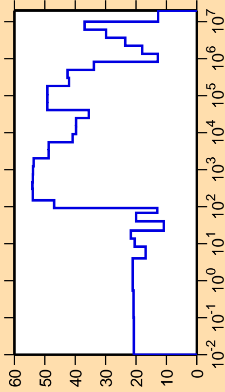
\Delta\sigma/\sigma vs. E for ^{185}\text{Hf}(n,\text{el.})
