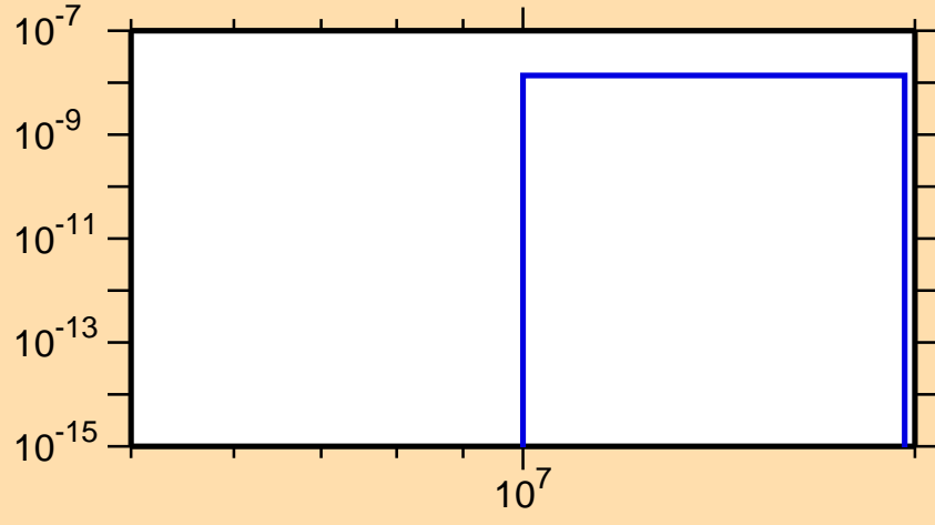
\sigma vs. E for ^{185}\text{Hf}(n,2n\alpha)
