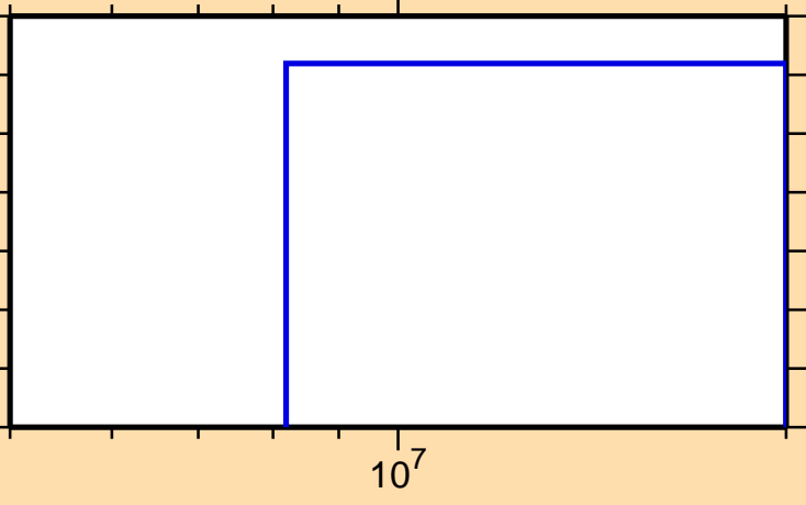
\sigma vs. E for ^{185}\text{Hf}(n,d)
