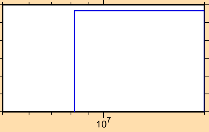
\sigma vs. E for ^{185}\text{Hf}(n,2n\alpha)
