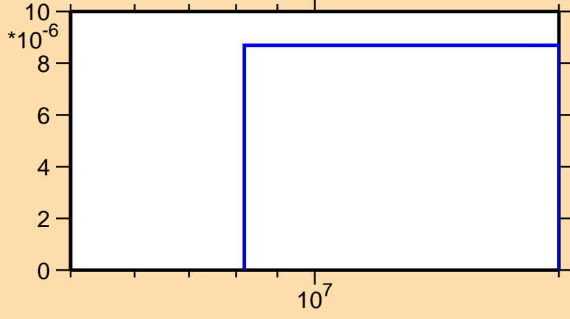
\sigma vs. E for ^{185}\text{Hf}(n,np)
