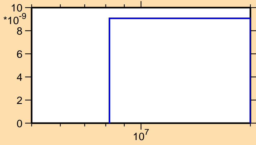
\sigma vs. E for ^{186}\text{Hf}(n,2n\alpha)
