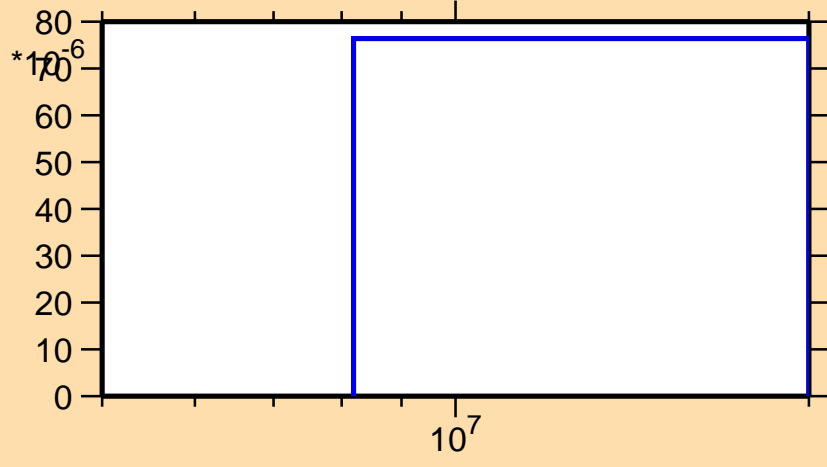
\sigma vs. E for ^{186}\text{Hf}(n,p)
