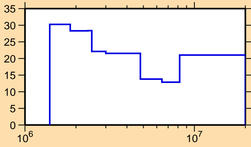
\Delta\sigma/\sigma vs. E for ^{186}\text{Hf}(n,\text{el.})
