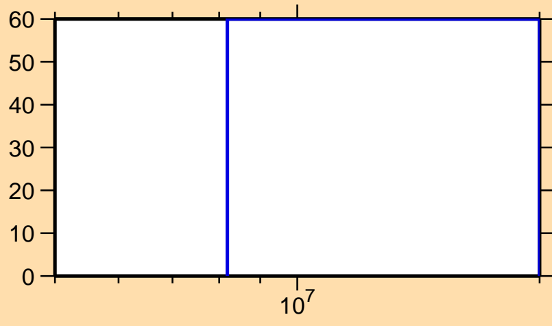
\Delta\sigma/\sigma vs. E for ^{186}\text{Hf}(n,p)
