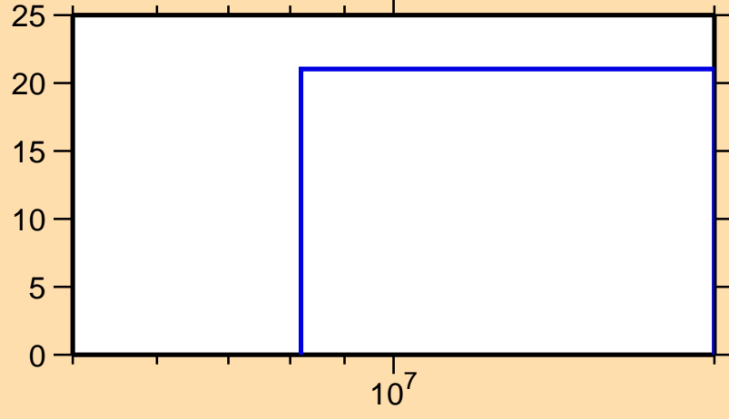
\Delta\sigma/\sigma vs. E for ^{186}\text{Hf}(n,el.)
