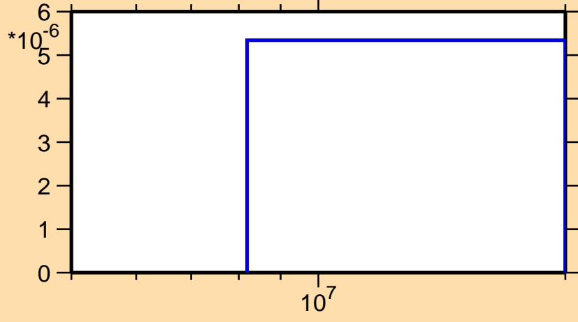
\sigma vs. E for ^{186}\text{Hf}(n,d)
