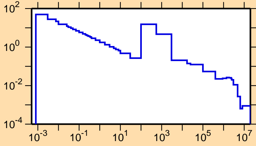
\sigma vs. E for ^{186}\text{Hf}(n,\gamma)
