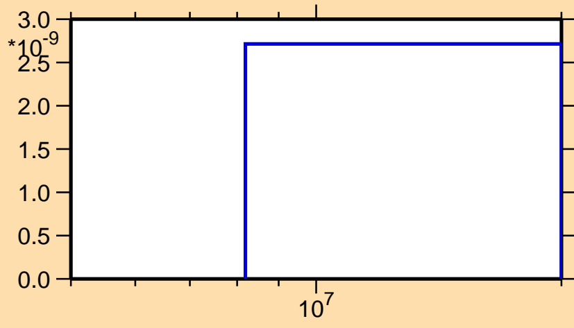
\sigma vs. E for ^{186}\text{Hf}(n,nt)
