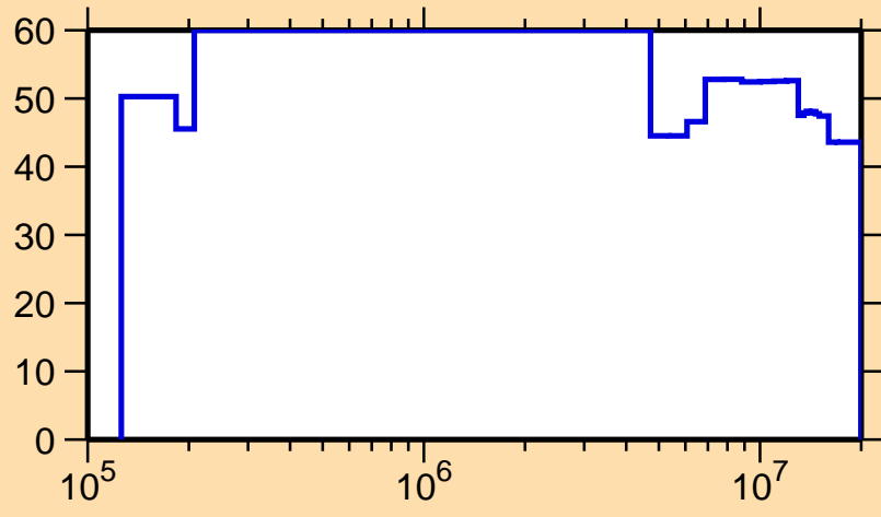
\Delta\sigma/\sigma vs. E for ^{187}\text{Hf}(n,n_1)
