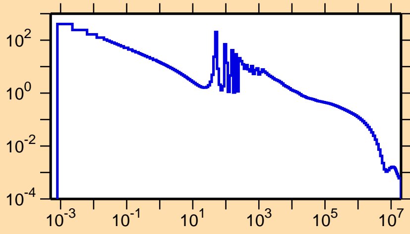
\sigma vs. E for ^{187}\text{Hf}(n,\gamma)
