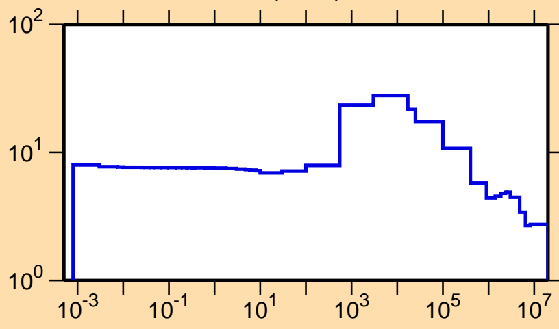
\sigma vs. E for ^{187}\text{Hf}(n,\text{el.})
