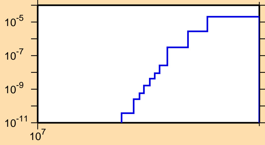
\sigma vs. E for ^{188}\text{Hf}(n,t)
