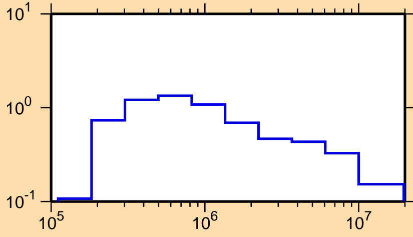
\sigma vs. E for ^{188}\text{Hf}(n,n_1)
