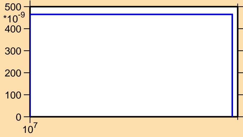
\sigma vs. E for ^{188}\text{Hf}(n,np)
