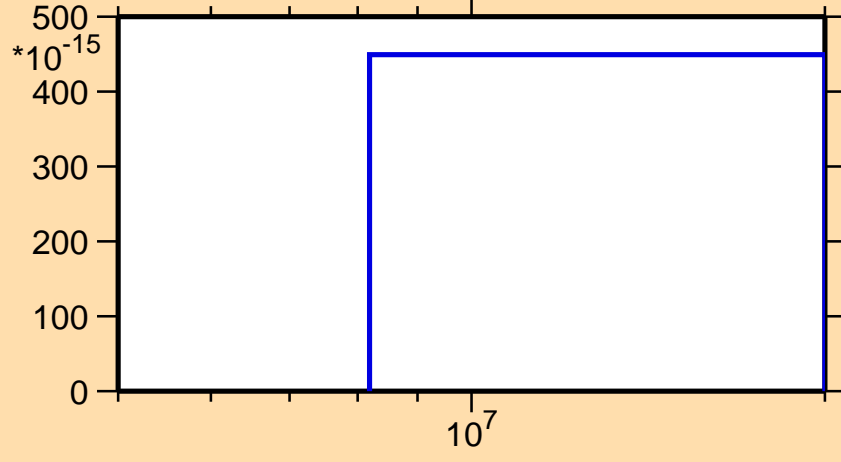
\sigma vs. E for ^{188}\text{Hf}(n,nd)
