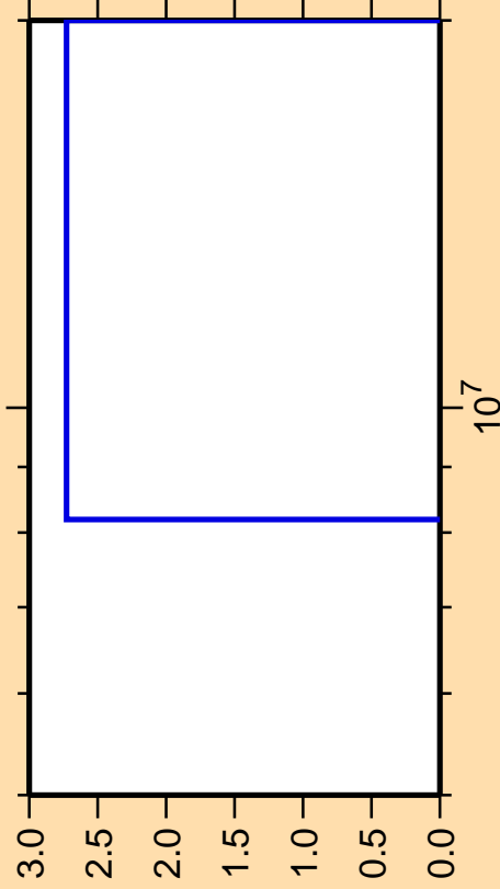
\Delta\sigma/\sigma vs. E for ^{188}\text{Hf}(n,nd)
