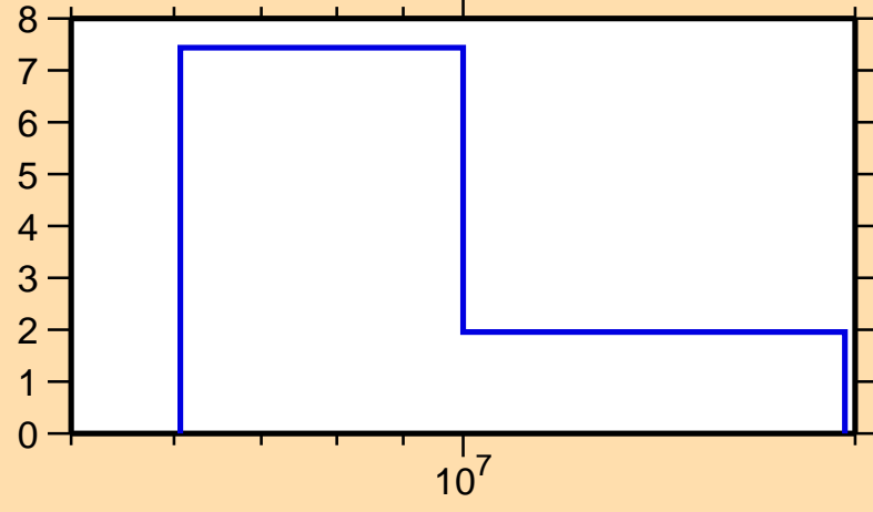
\Delta\sigma/\sigma vs. E for ^{189}\text{Hf}(n,\text{tot.})
