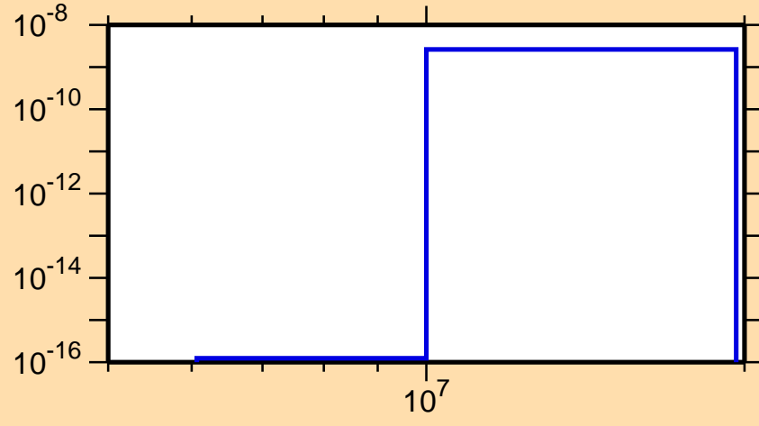
\sigma vs. E for ^{189}\text{Hf}(n,2n\alpha)
