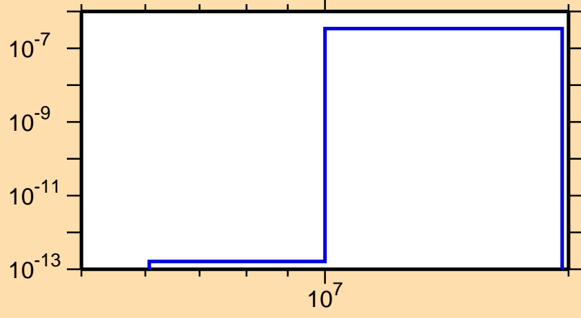
\sigma vs. E for ^{189}\text{Hf}(n,n\alpha)
