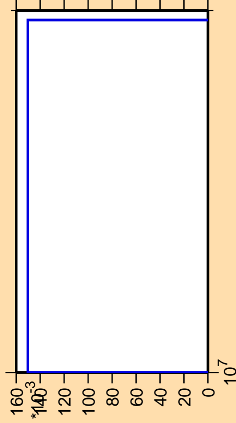
\Delta\sigma/\sigma vs. E for ^{189}\text{Hf}(n,3n\alpha)
