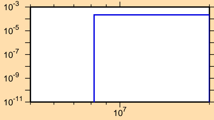
\sigma vs. E for ^{189}\text{Hf}(n,p)
