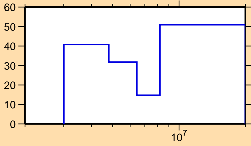
\Delta\sigma/\sigma vs. E for ^{189}\text{Hf}(n,2n)
