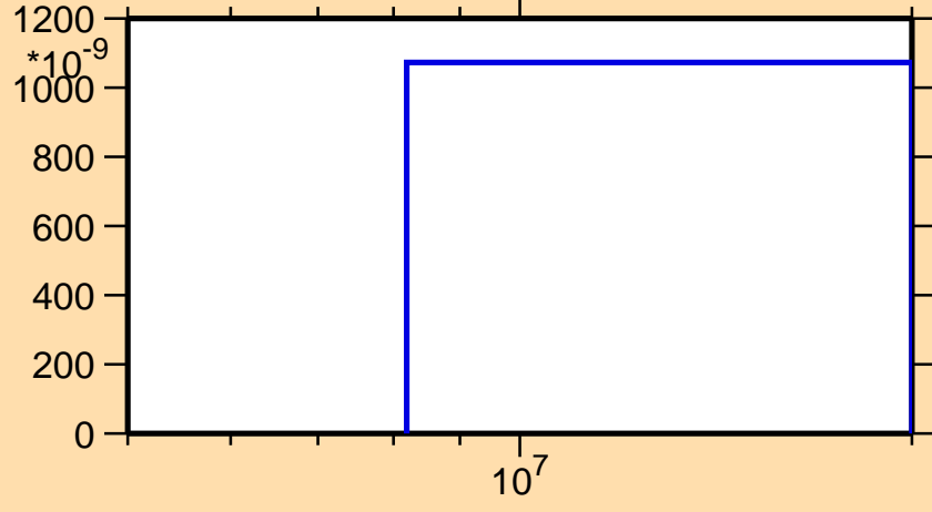
\sigma vs. E for ^{189}\text{Hf}(n,d)
