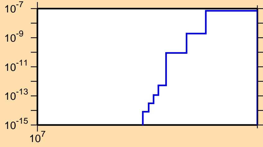
\sigma vs. E for ^{180}\text{Hg}(n,\text{nd})
