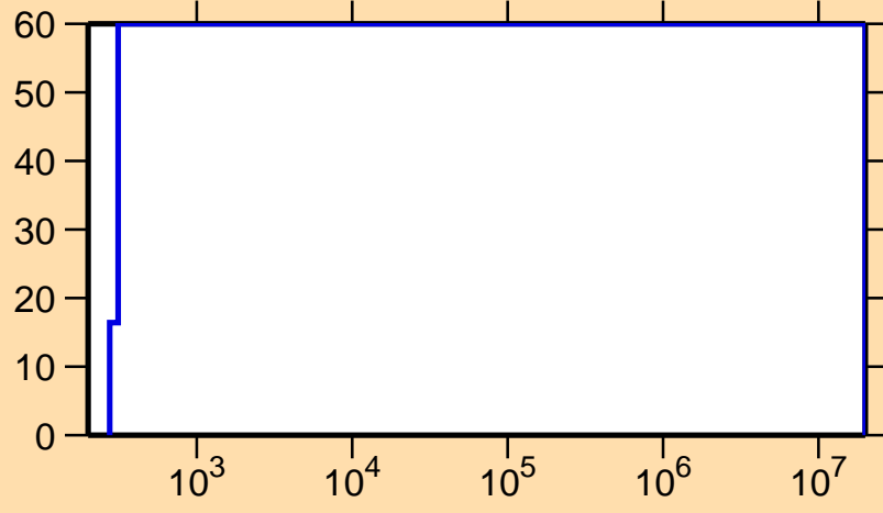
\Delta\sigma/\sigma vs. E for ^{180}\text{Hg}(n,\gamma)
