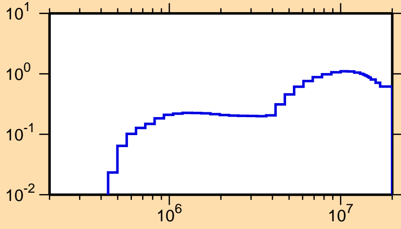
\sigma vs. E for ^{180}\text{Hg}(n,\text{inel.})
