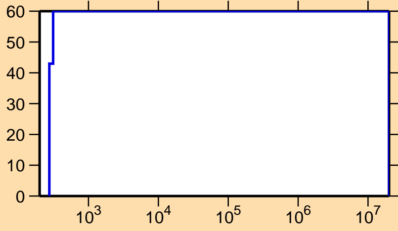
\Delta\sigma/\sigma vs. E for ^{180}\text{Hg}(n,p)
