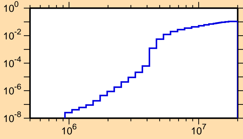
\sigma vs. E for ^{180}\text{Hg}(n,n\alpha)
