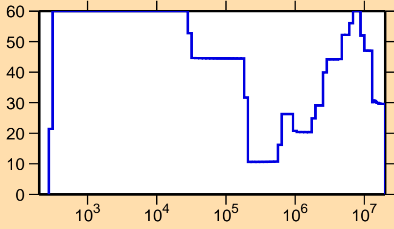
\Delta\sigma/\sigma vs. E for ^{180}\text{Hg}(n,\text{el.})
