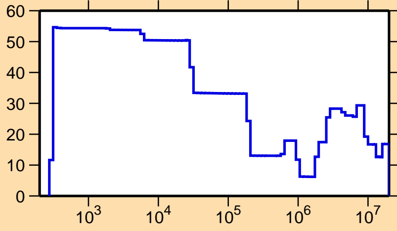
\Delta\sigma/\sigma vs. E for ^{180}\text{Hg}(n,\text{tot.})
