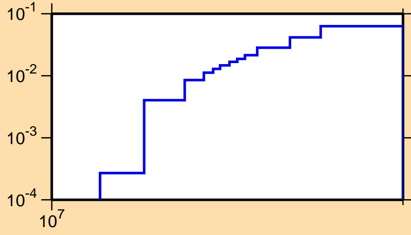
\sigma vs. E for ^{180}\text{Hg}(n,2n)
