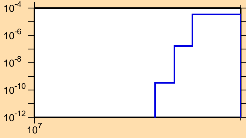
\sigma vs. E for ^{180}\text{Hg}(n,2np)
