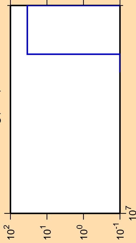
\Delta\sigma/\sigma vs. E for ^{180}\text{Hg}(n,nt)
