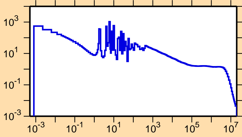
\sigma vs. E for ^{180}\text{Hg}(n,\gamma)
