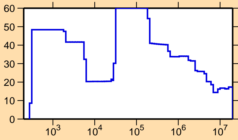
\Delta\sigma/\sigma vs. E for ^{180}\text{Hg}(n,\text{nonel.})
