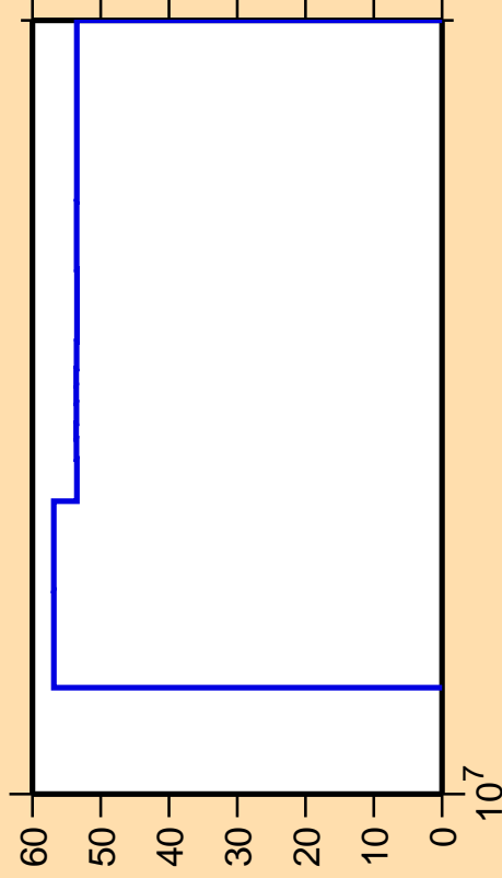
\Delta\sigma/\sigma vs. E for ^{180}\text{Hg}(n,n_1)
