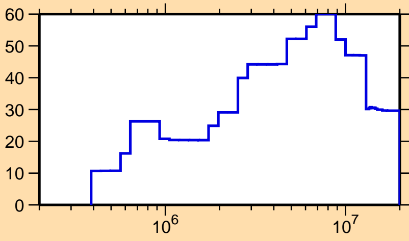
\Delta\sigma/\sigma vs. E for ^{180}\text{Hg}(n,\text{el.})
