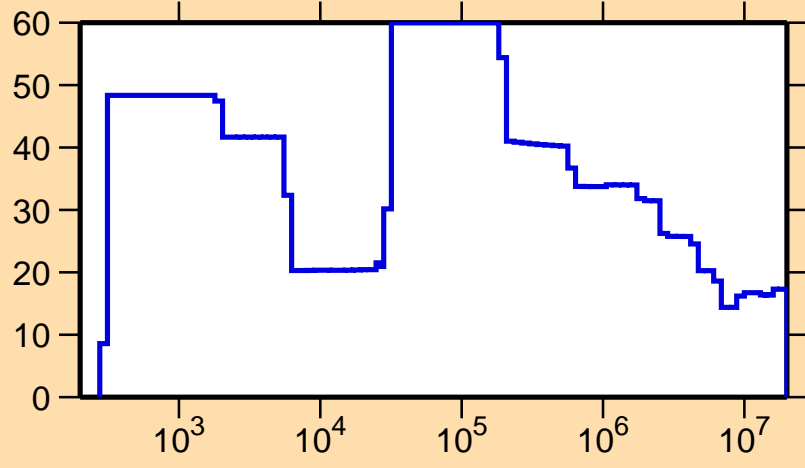
\Delta\sigma/\sigma vs. E for ^{180}\text{Hg}(n,\text{nonel.})
