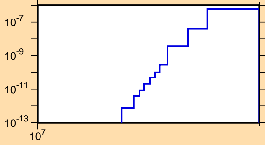
\sigma vs. E for ^{180}\text{Hg}(n,\text{pt})
