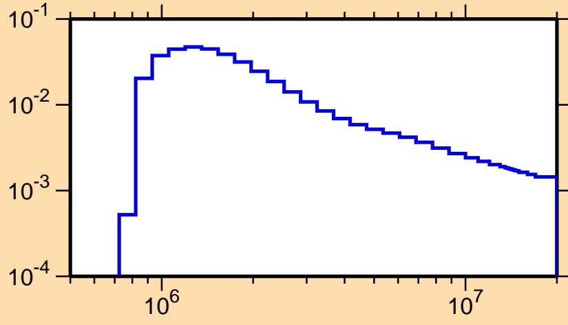
\sigma vs. E for ^{180}\text{Hg}(n,n_3)
