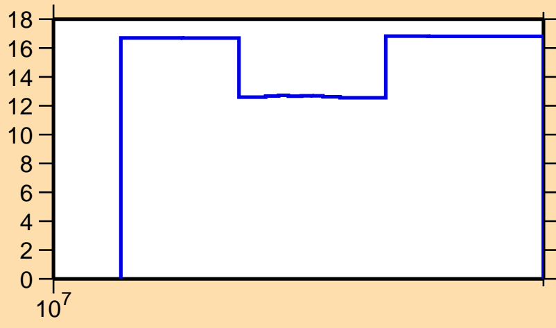
\Delta\sigma/\sigma vs. E for ^{180}\text{Hg}(n,\text{tot.})
