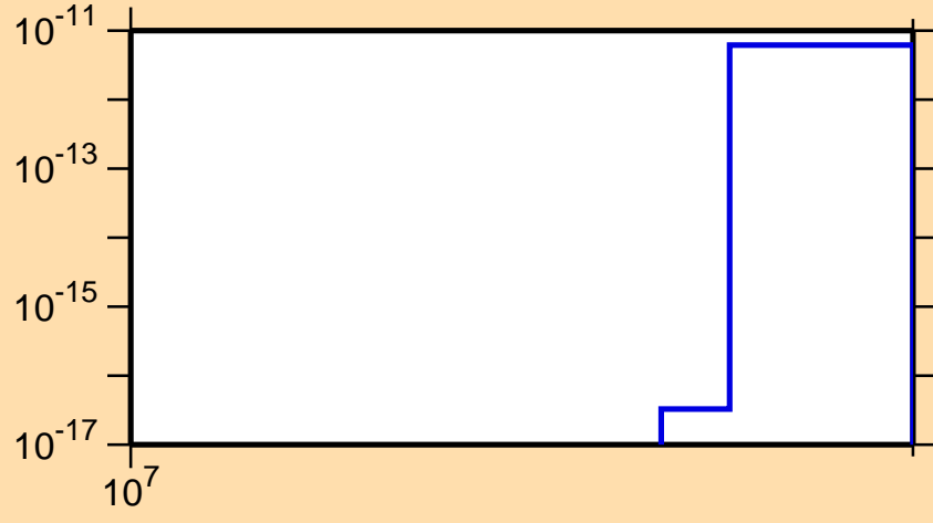
\sigma vs. E for ^{180}\text{Hg}(n,nt)
