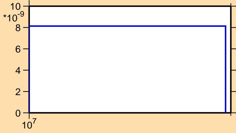
\sigma vs. E for ^{180}\text{Hg}(n,\text{pt})
