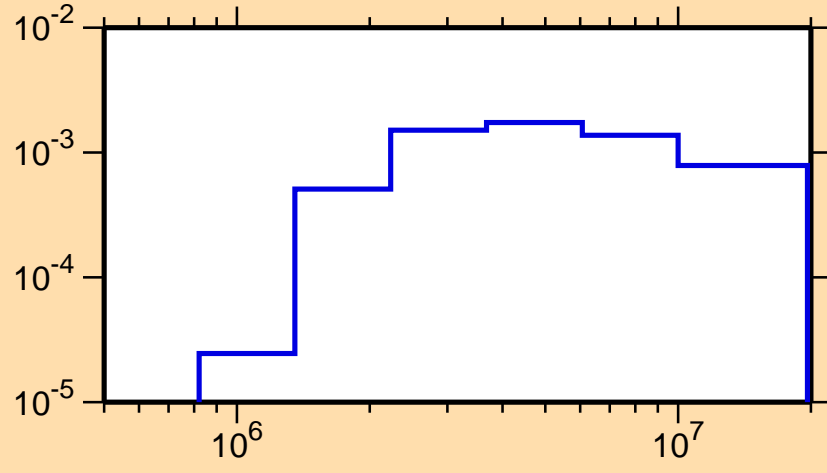
\sigma vs. E for ^{180}\text{Hg}(n,n_4)
