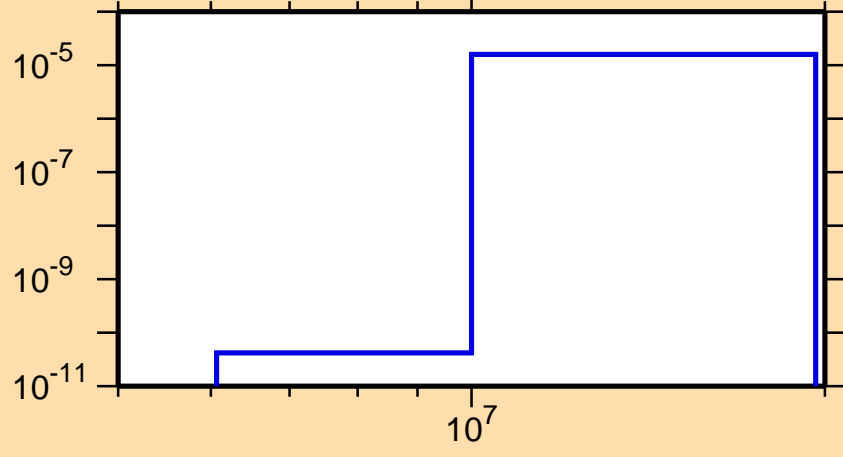
\sigma vs. E for ^{180}\text{Hg}(n,\text{pd})
