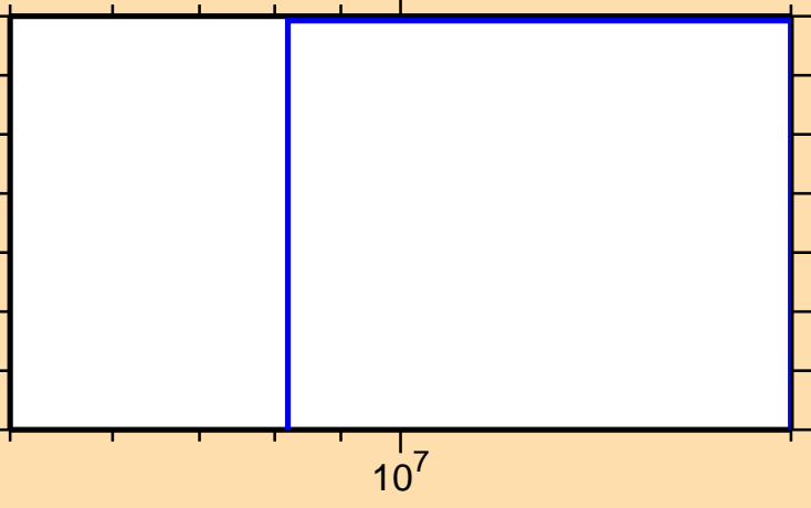
\sigma vs. E for ^{180}\text{Hg}(n,\text{pt})
