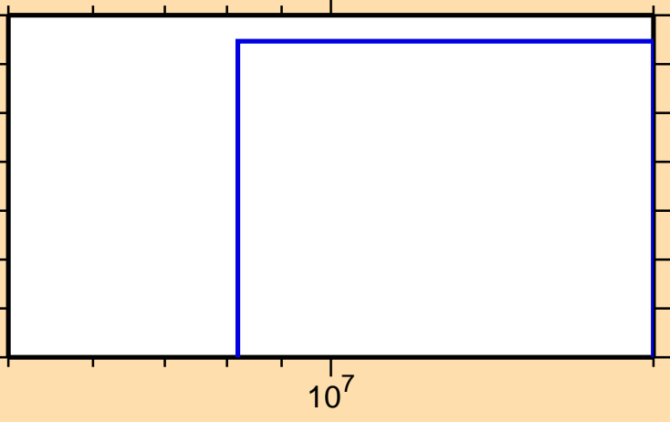
\sigma vs. E for ^{180}\text{Hg}(n,t)
