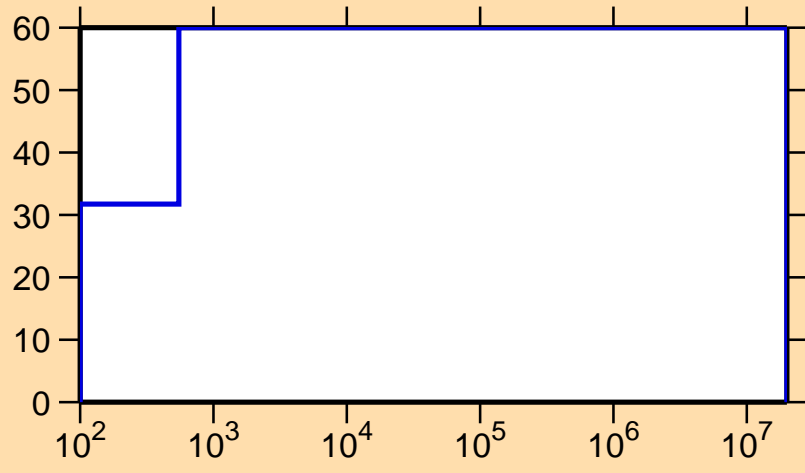
\Delta\sigma/\sigma vs. E for ^{180}\text{Hg}(n,\gamma)
