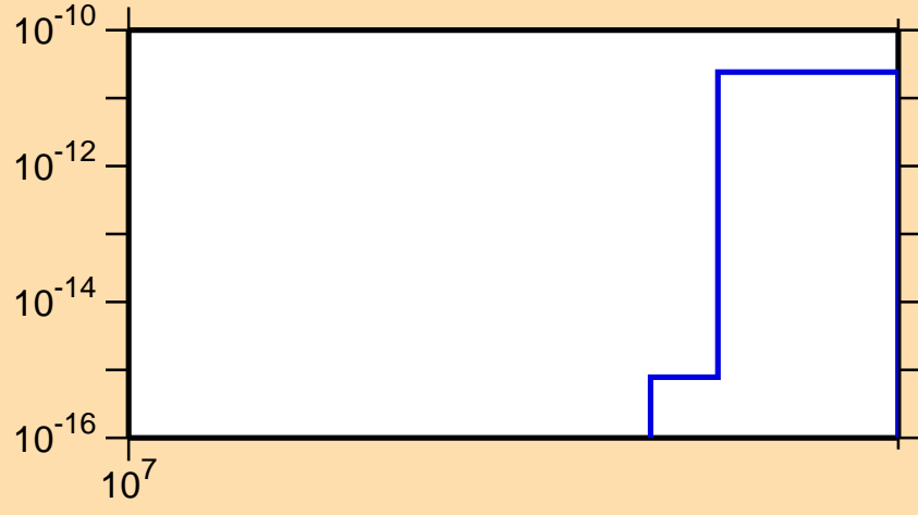
\sigma vs. E for ^{181}\text{Hg}(n,nt)
