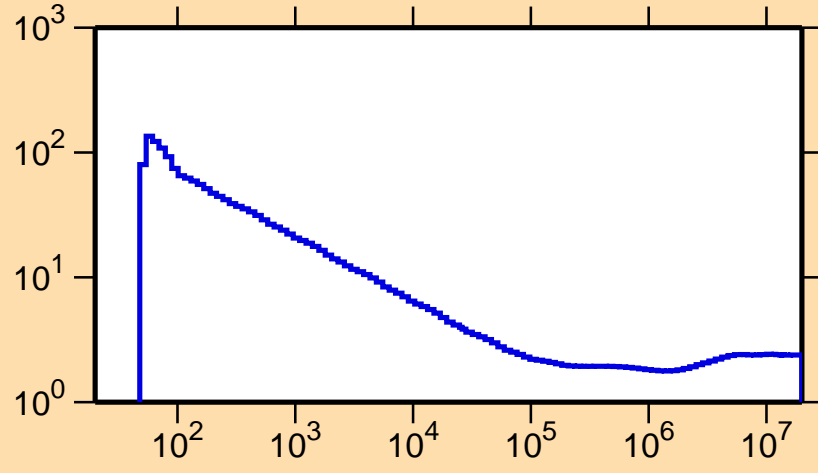
\sigma vs. E for ^{181}\text{Hg}(n,\text{nonel.})
