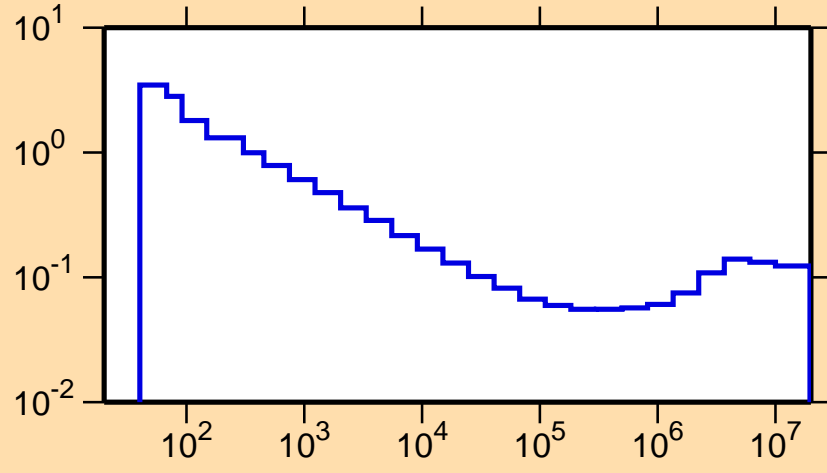
\sigma vs. E for ^{181}\text{Hg}(n,\alpha)
