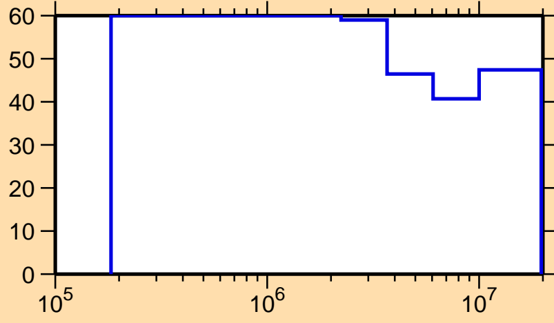
\Delta\sigma/\sigma vs. E for ^{181}\text{Hg}(n,n\text{cont.})
