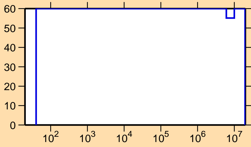
\Delta\sigma/\sigma vs. E for ^{181}\text{Hg}(n,p)
