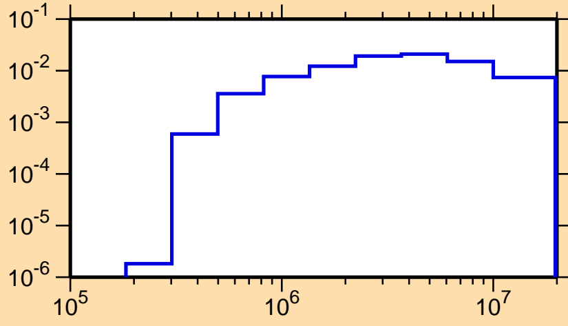
\sigma vs. E for ^{181}\text{Hg}(n,n_3)
