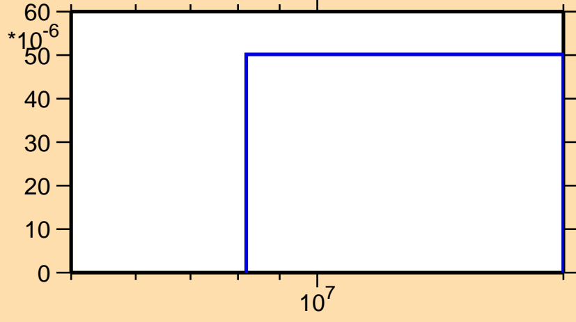
\sigma vs. E for ^{181}\text{Hg}(n,2np)
