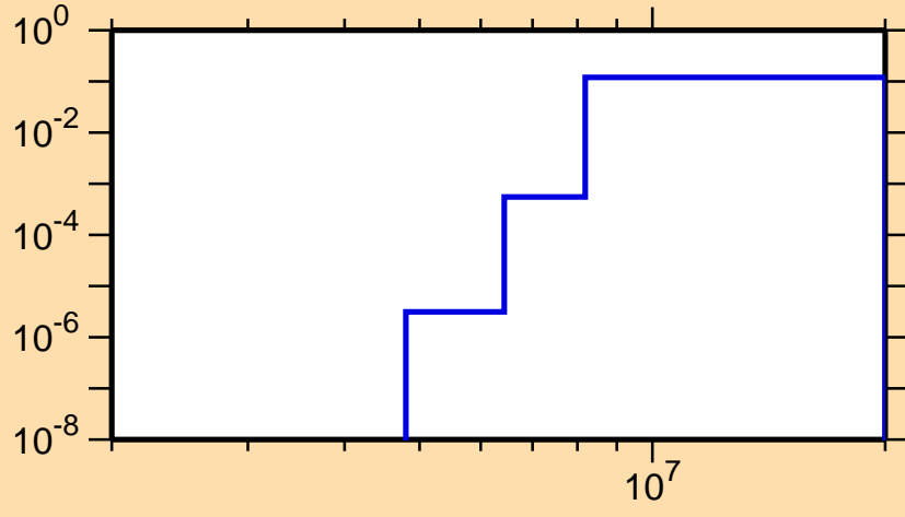
\sigma vs. E for ^{181}\text{Hg} (mt 45)
