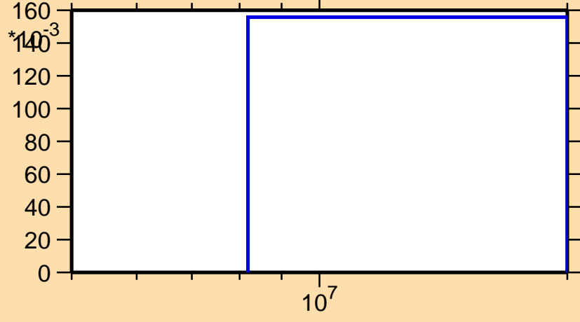
\sigma vs. E for ^{181}\text{Hg}(n,2n)
