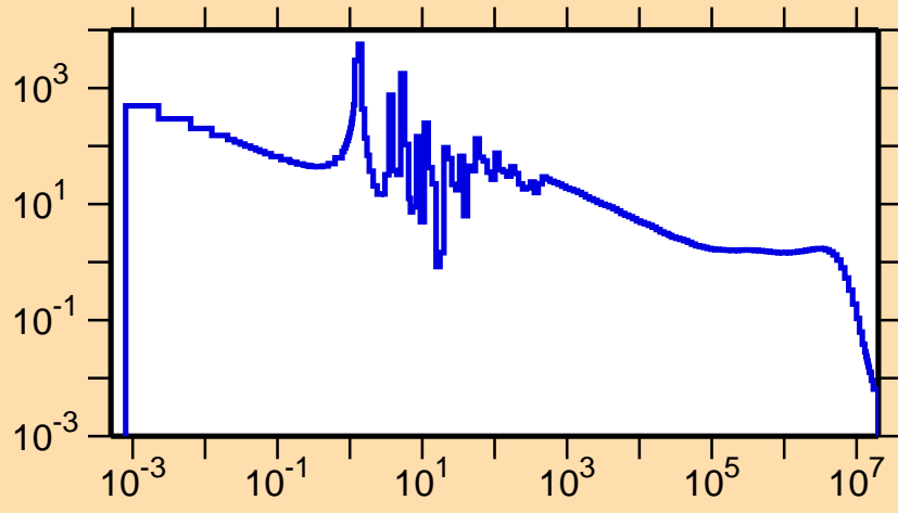
\sigma vs. E for ^{182}\text{Hg}(n,\gamma)
