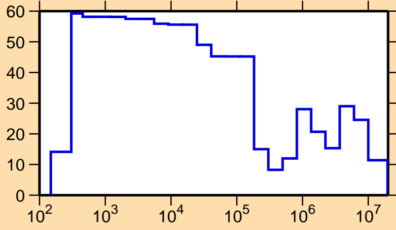
\Delta\sigma/\sigma vs. E for ^{182}\text{Hg}(n,\text{el.})
