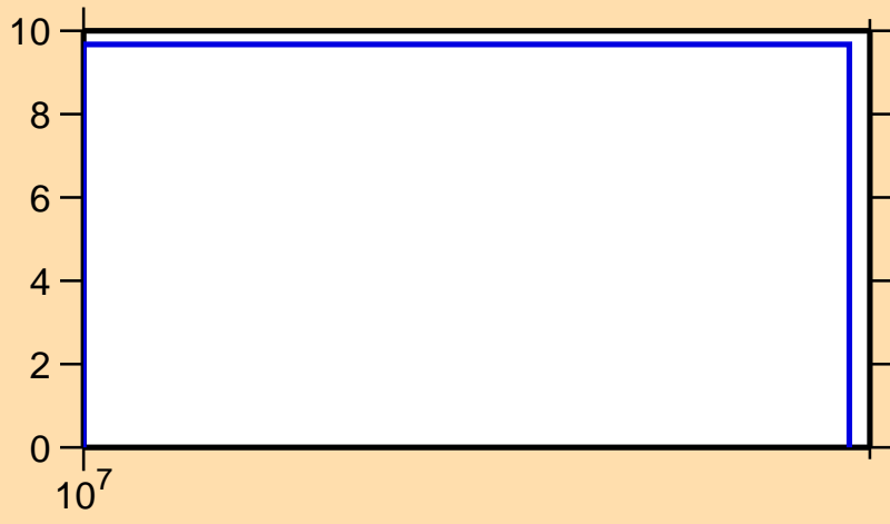
\Delta\sigma/\sigma vs. E for ^{182}\text{Hg}(n,\text{tot.})
