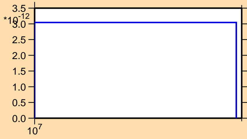
\sigma vs. E for ^{182}\text{Hg} (mt 34)
