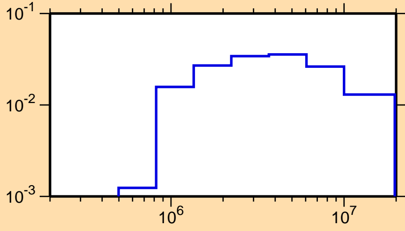
\sigma vs. E for ^{182}\text{Hg}(n,n_4)
