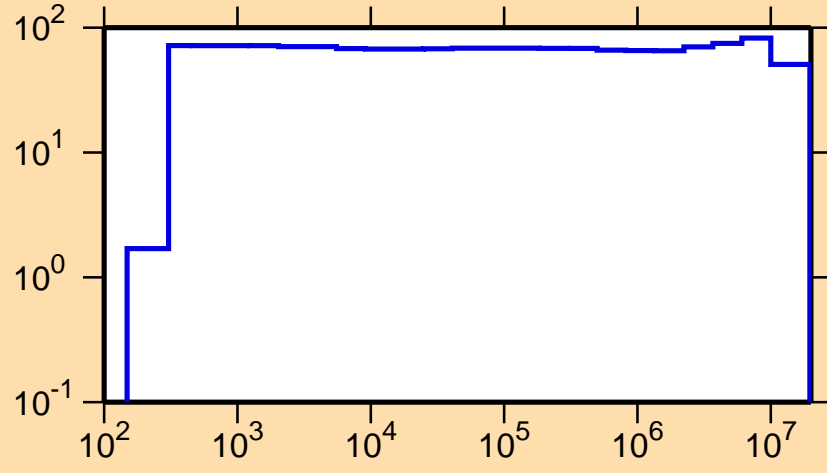
\Delta\sigma/\sigma vs. E for ^{182}\text{Hg}(n,\gamma)
