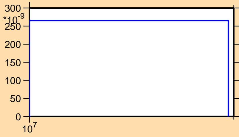
\sigma vs. E for ^{182}\text{Hg}(n,2np)
