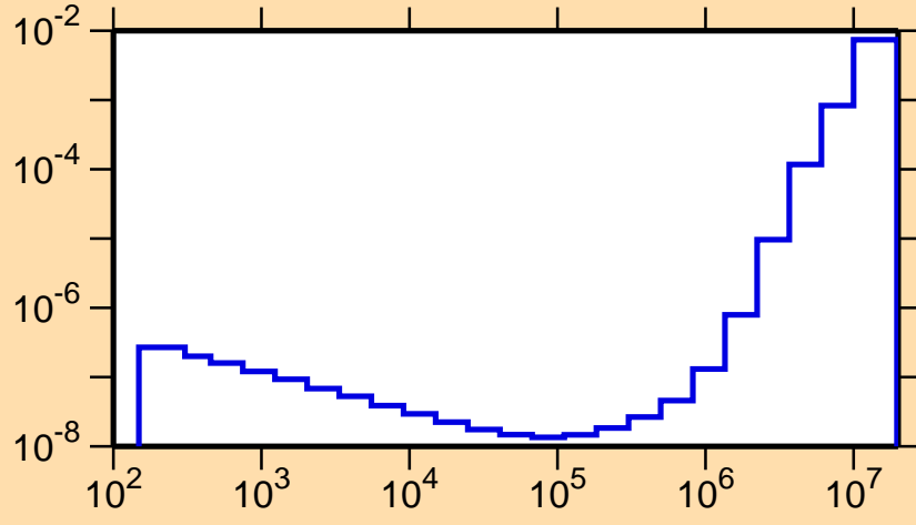
\sigma vs. E for ^{182}\text{Hg}(n,p\alpha)
