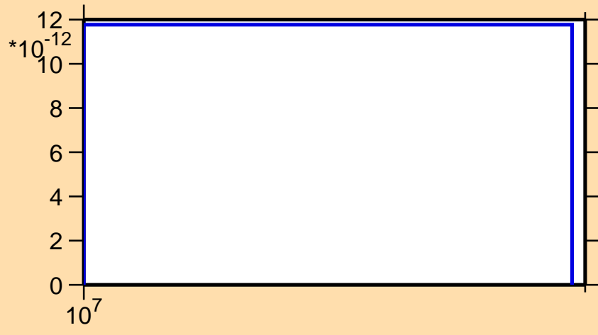
\sigma vs. E for ^{182}\text{Hg}(n,3n)
