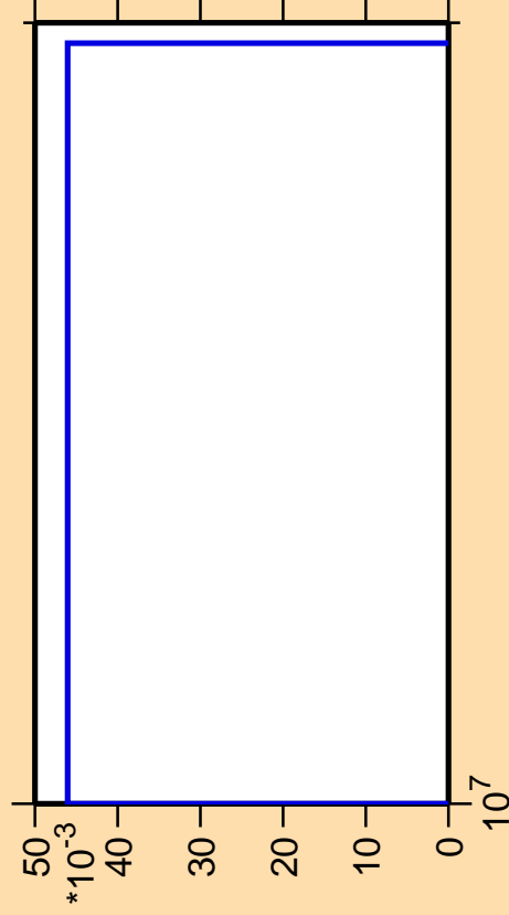
\Delta\sigma/\sigma vs. E for ^{182}\text{Hg}(n,nt)
