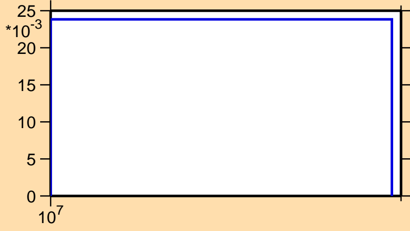
\sigma vs. E for ^{182}\text{Hg}(n,2n)
