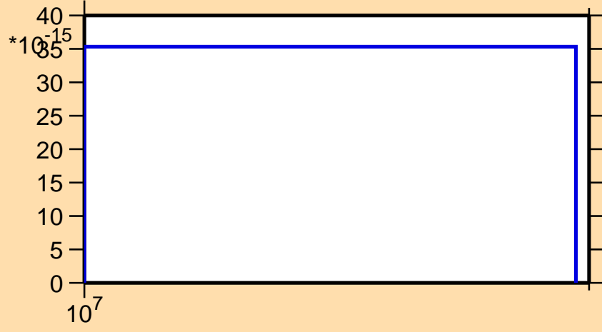
\sigma vs. E for ^{182}\text{Hg}(n,nt)
