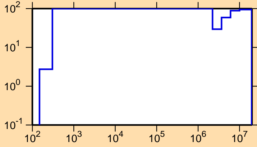
\Delta\sigma/\sigma vs. E for ^{182}\text{Hg}(n,p)
