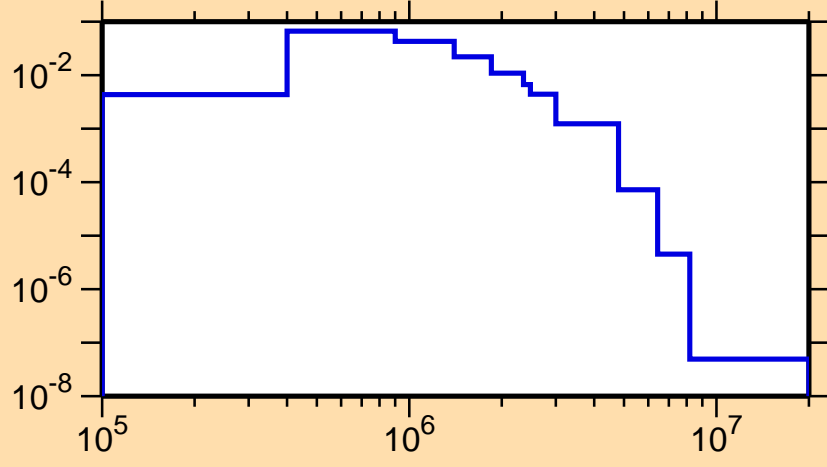
\sigma vs. E for ^{182}\text{Hg}(n,n_1)
