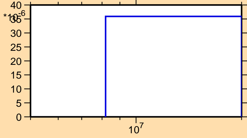
\sigma vs. E for ^{182}\text{Hg}(n,t)
