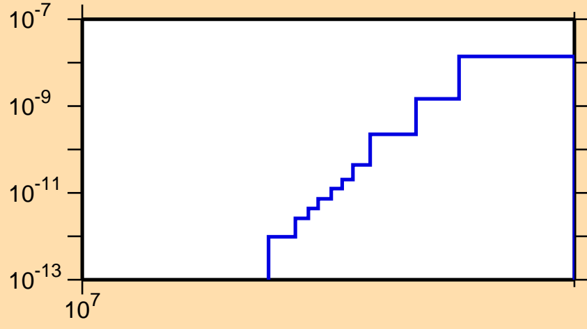
\sigma vs. E for ^{183}\text{Hg} (mt 34)
