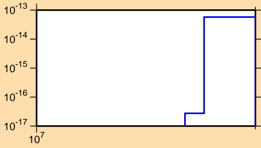
\sigma vs. E for ^{183}\text{Hg}(n,3n\alpha)
