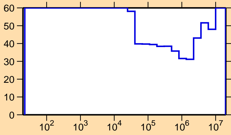
\Delta\sigma/\sigma vs. E for ^{183}\text{Hg}(n,\gamma)
