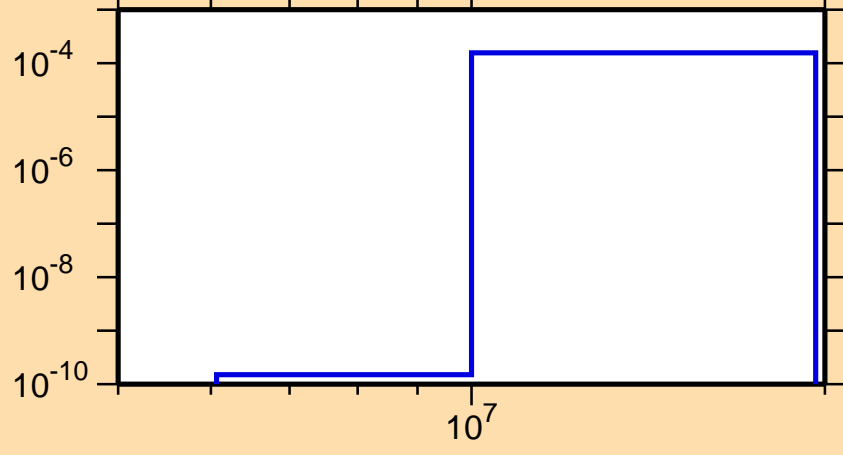
\sigma vs. E for ^{183}\text{Hg}(n,t)
