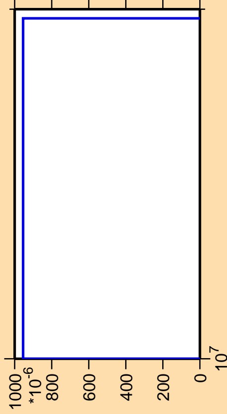
\Delta\sigma/\sigma vs. E for ^{183}\text{Hg}(n,3n\alpha)
