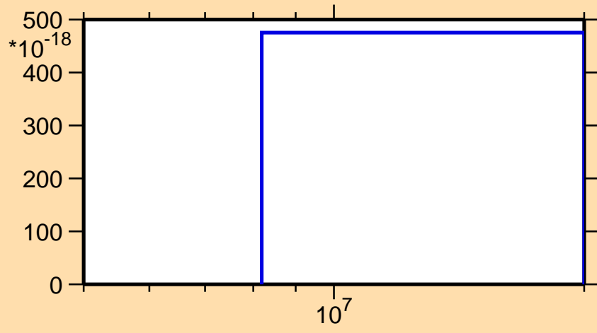
\sigma vs. E for ^{183}\text{Hg}(n,3n\alpha)
