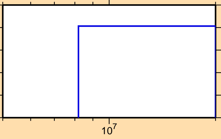
\sigma vs. E for ^{183}\text{Hg} (mt 34)
