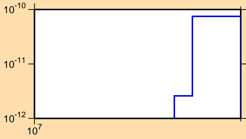
\sigma vs. E for ^{184}\text{Hg} (mt 34)
