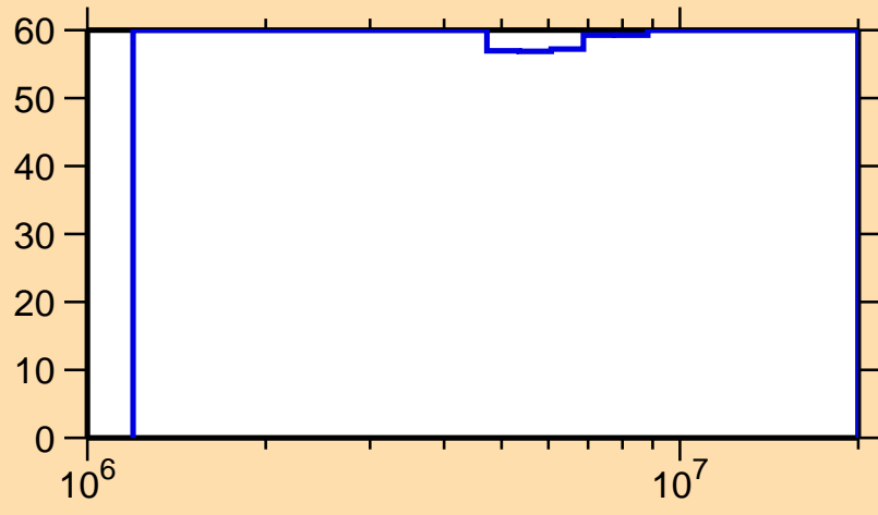
\Delta\sigma/\sigma vs. E for ^{184}\text{Hg}(n,n\text{cont.})
