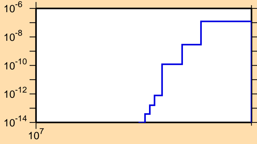
\sigma vs. E for ^{184}\text{Hg}(n,\text{nd})
