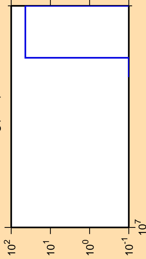
\Delta\sigma/\sigma vs. E for ^{184}\text{Hg}(n,nt)
