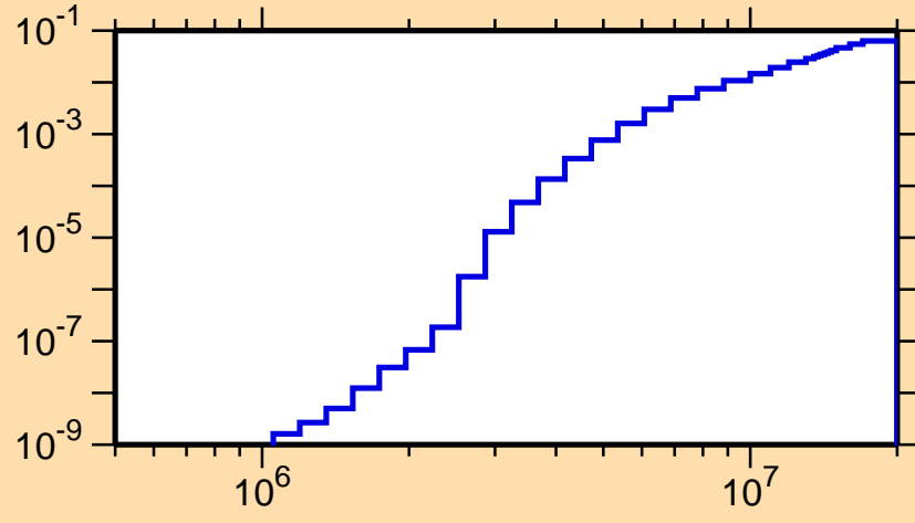
\sigma vs. E for ^{184}\text{Hg}(n,n\alpha)
