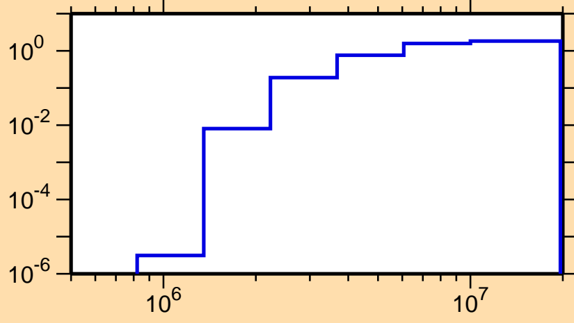
\sigma vs. E for ^{184}\text{Hg}(n,n\text{cont.})
