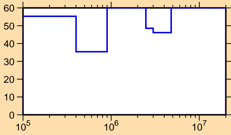
\Delta\sigma/\sigma vs. E for ^{184}\text{Hg}(n,n_1)
