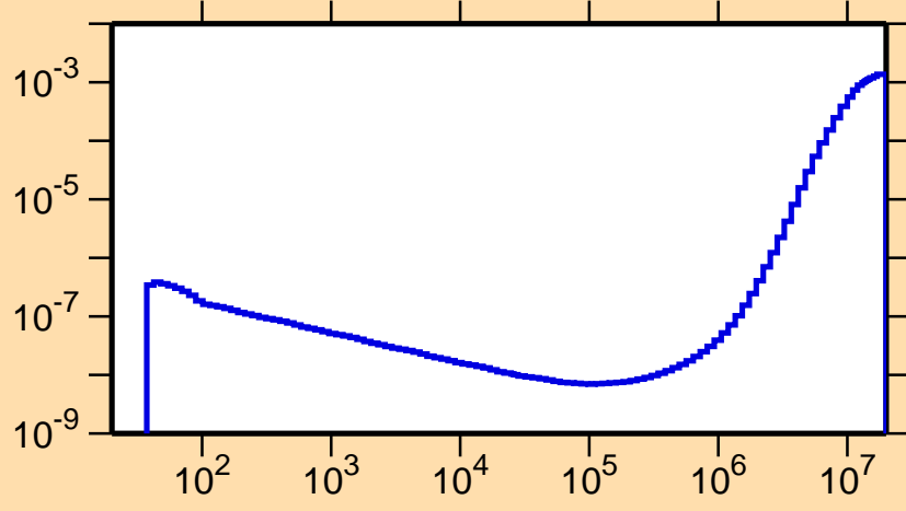
\sigma vs. E for ^{185}\text{Hg}(n,p\alpha)
