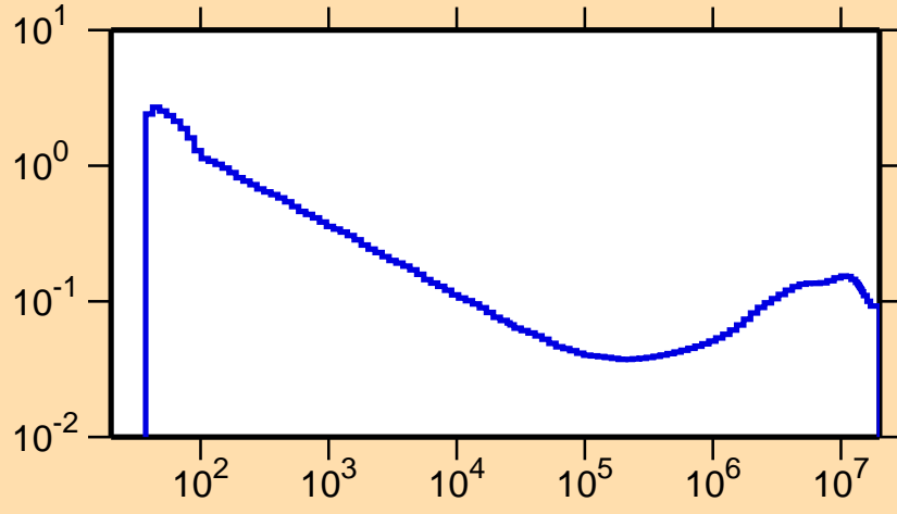
\sigma vs. E for ^{185}\text{Hg}(n,p)
