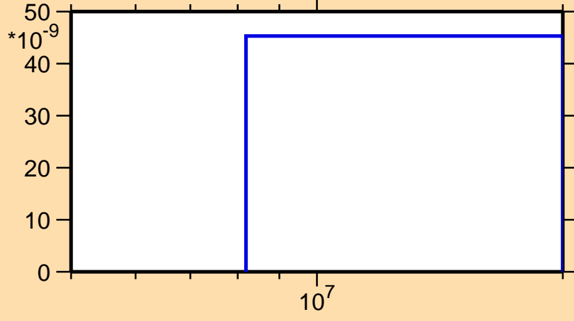
\sigma vs. E for ^{185}\text{Hg}(n,\text{pd})
