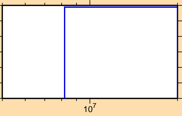
\sigma vs. E for ^{185}\text{Hg}(\text{mt117})
