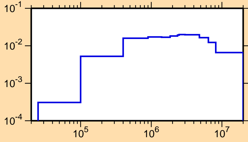
\sigma vs. E for ^{185}\text{Hg}(n,n_2)
