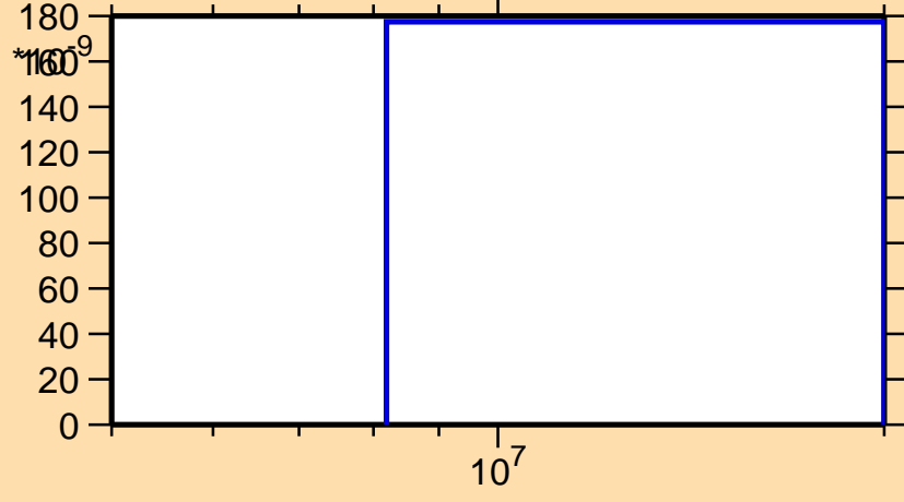
\sigma vs. E for ^{185}\text{Hg}(n,3n)
