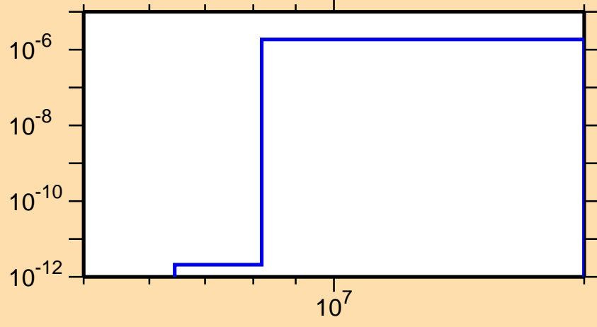
\sigma vs. E for ^{185}\text{Hg}(n,\text{He}3)
