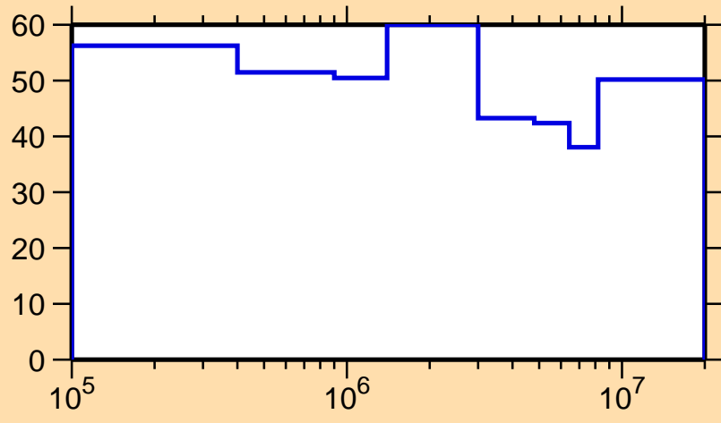
\Delta\sigma/\sigma vs. E for ^{185}\text{Hg}(n,n\text{cont.})
