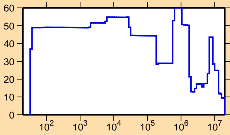
\Delta\sigma/\sigma vs. E for ^{185}\text{Hg}(n,\text{tot.})
