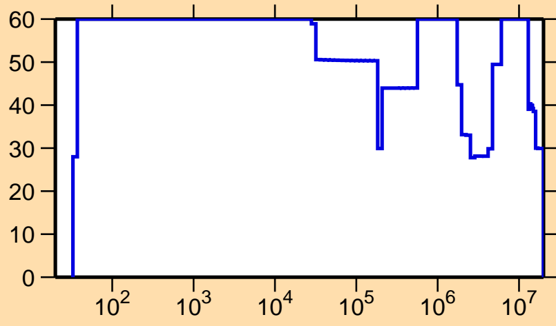
\Delta\sigma/\sigma vs. E for ^{185}\text{Hg}(n,\text{el.})
