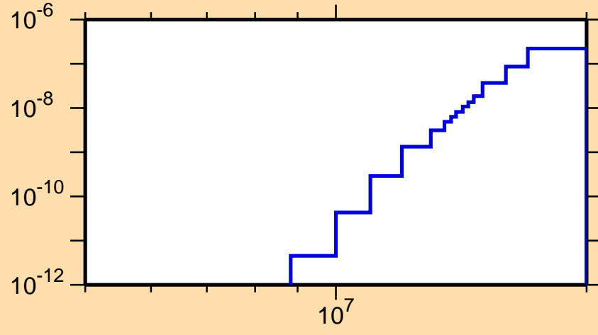
\sigma vs. E for ^{185}\text{Hg}(\text{mt117})
