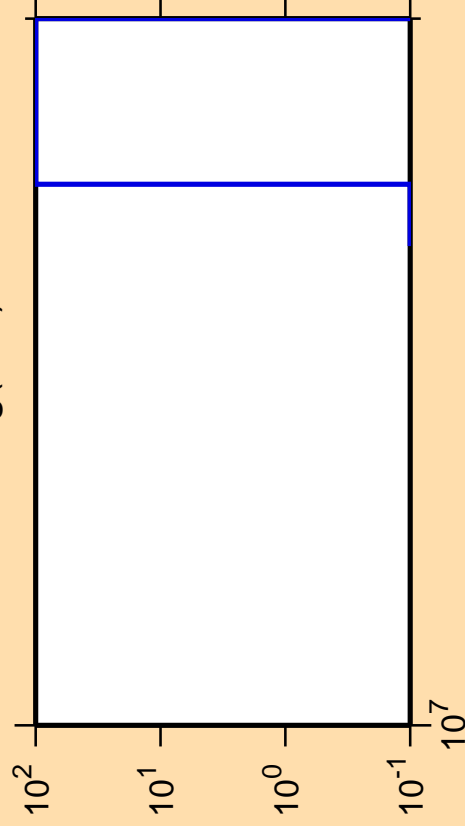
\Delta\sigma/\sigma vs. E for ^{185}\text{Hg}(n,nt)
