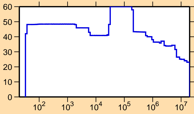
\Delta\sigma/\sigma vs. E for ^{185}\text{Hg}(n,\text{nonel.})
