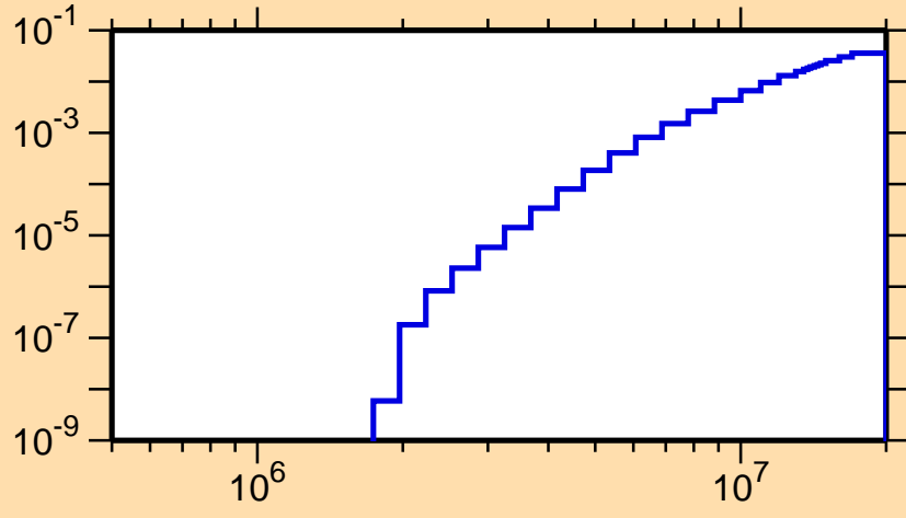
\sigma vs. E for ^{185}\text{Hg}(n,n\alpha)
