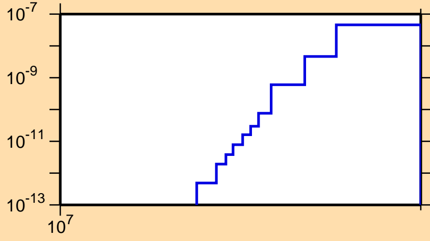
\sigma vs. E for ^{185}\text{Hg}(n,\text{pt})
