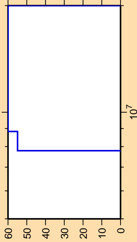
\Delta\sigma/\sigma vs. E for ^{185}\text{Hg}(n,n\text{cont.})
