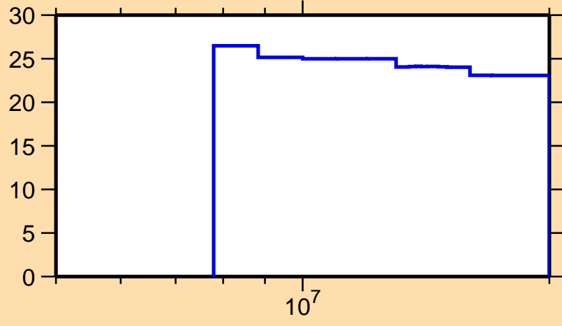
\Delta\sigma/\sigma vs. E for ^{185}\text{Hg}(n,\text{nonel.})
