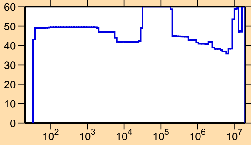
\Delta\sigma/\sigma vs. E for ^{185}\text{Hg}(n,\gamma)
