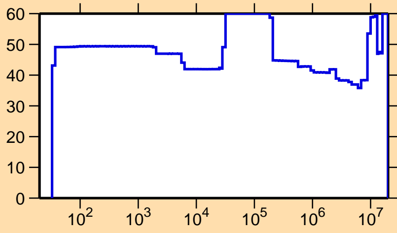
\Delta\sigma/\sigma vs. E for ^{185}\text{Hg}(n,\gamma)
