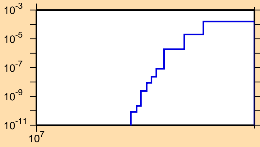
\sigma vs. E for ^{185}\text{Hg}(n,2np)
