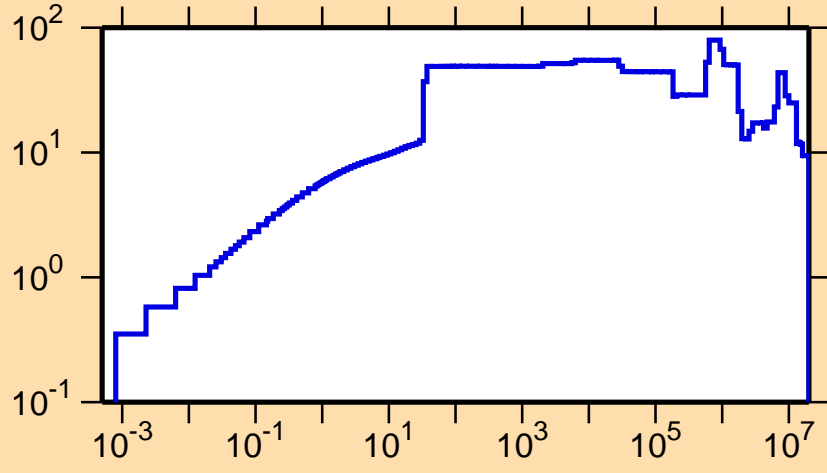
\Delta\sigma/\sigma vs. E for ^{185}\text{Hg}(n,\text{tot.})
