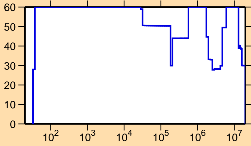
\Delta\sigma/\sigma vs. E for ^{185}\text{Hg}(n,\text{el.})
