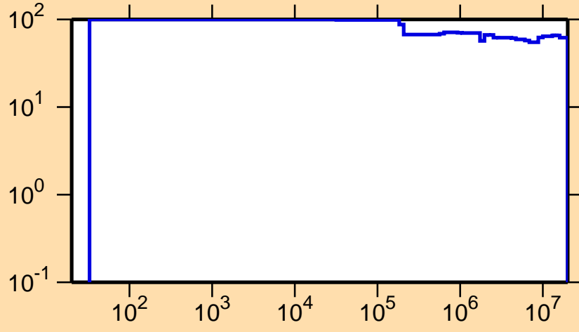
\Delta\sigma/\sigma vs. E for ^{185}\text{Hg}(n,n\text{cont.})
