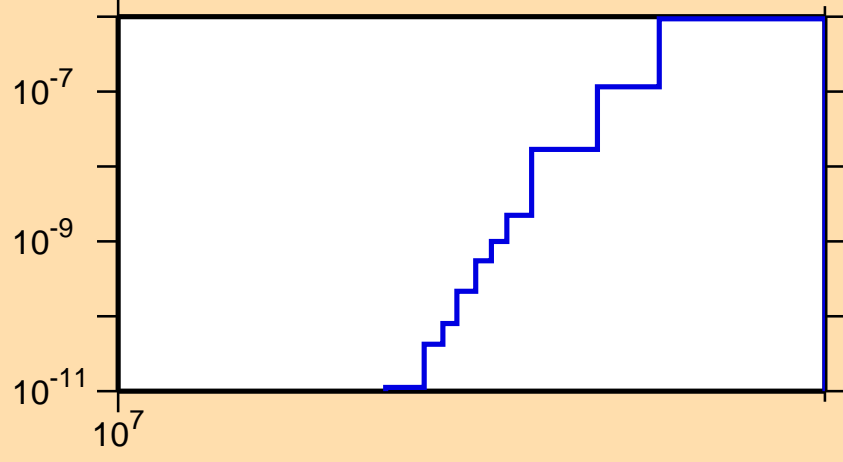
\sigma vs. E for ^{185}\text{Hg}(n,\text{nd})
