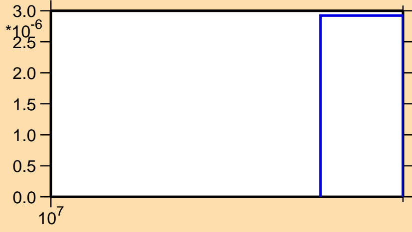
\sigma vs. E for ^{185}\text{Hg}(n,3n)
