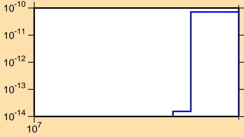
\sigma vs. E for ^{185}\text{Hg}(n,nt)
